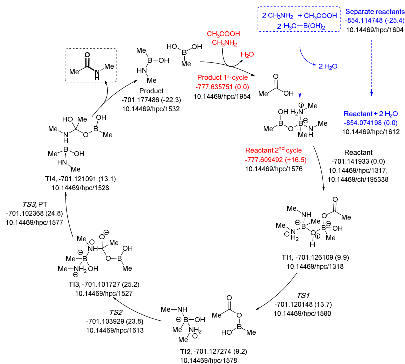
Figure 10. Catalytic cycle involving two amines (data 26 sub-collection DOI: 14469/hpc/1622; the labels have the same meaning as in Fig. 9).
