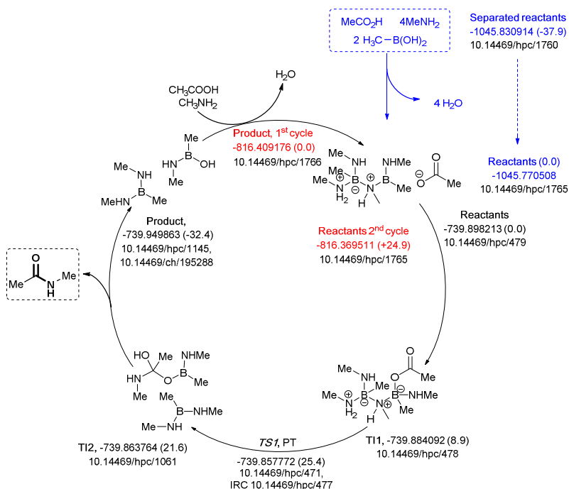
Figure 12. Catalytic cycle involving four amines (data 26 sub-collection DOI: 14469/hpc/1728; the labels have the same meaning as in Fig. 9).
