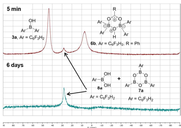
Figure 3. 11 B NMRs of a mixture of bis -3,4,5-trifluorophenylborinic acid 3a with benzoic acid after 5 min and after 6 days upon mixing (Ar = 3,4,5-trifluorophenyl).
