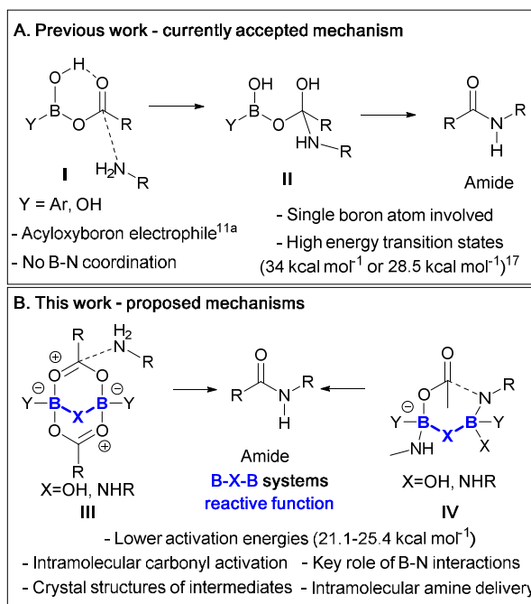
Scheme 2. A) Currently proposed mechanism via a monomeric acyloxyboron intermediate. B) Summary of mechanisms proposed in this paper involving dimeric B-X-B motifs.
