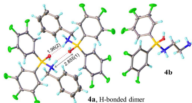
Figure 1. X-ray structures of Lewis adducts 4a (H-bonded dimer) and 4b .
