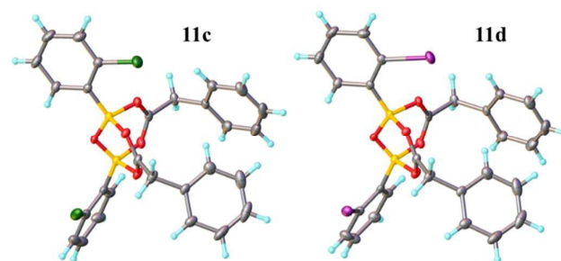
Figure 6. X-ray structures of B-O-B "ate"-complexes 11c and d .
