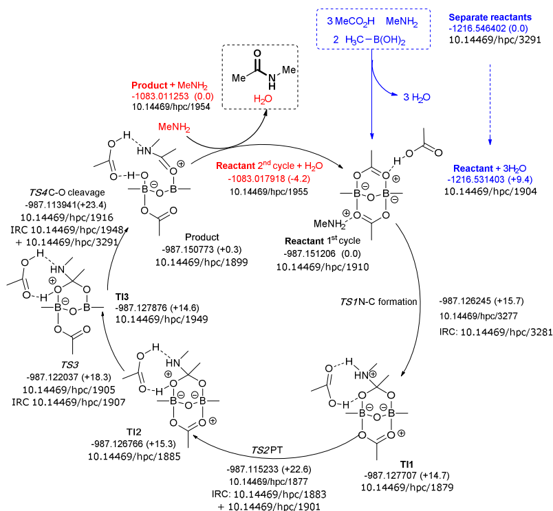
Figure 9. Catalytic cycle involving one amine (data 26 sub-collection DOI: 14469/hpc/1854). The total computed free energy for each stationary point is shown in Hartree, with the relative energies shown in parentheses in kcal mol -1 . The DOI for data repository entries for individual species are shown in the form e.g. 10.14469/hpc/1885. Energies in blue are for the pre-assembly stage, in black for the cycle proper and in red for the regeneration step to initiate a new cycle.
