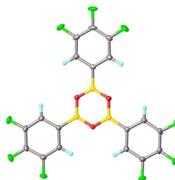
Figure 4. X-ray structure of 3,4,5-trifluorophenylboroxine 7a in orthorhombic \beta -form at 120 K.
