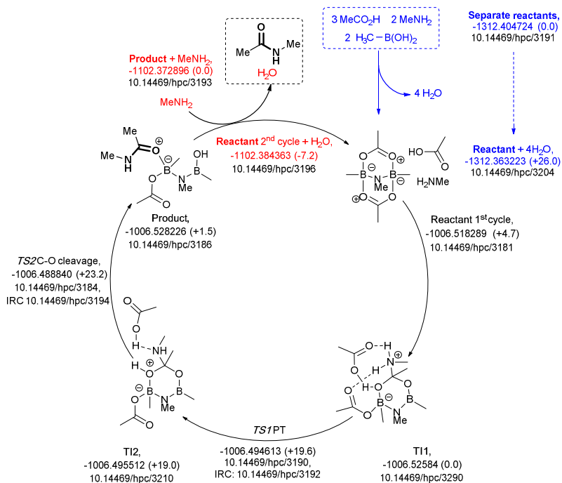
Figure 13. Catalytic cycle involving B-N-N bridging group (data 26 sub-collection DOI: 14469/hpc/3188; the labels have the same meaning as in Fig. 9).
