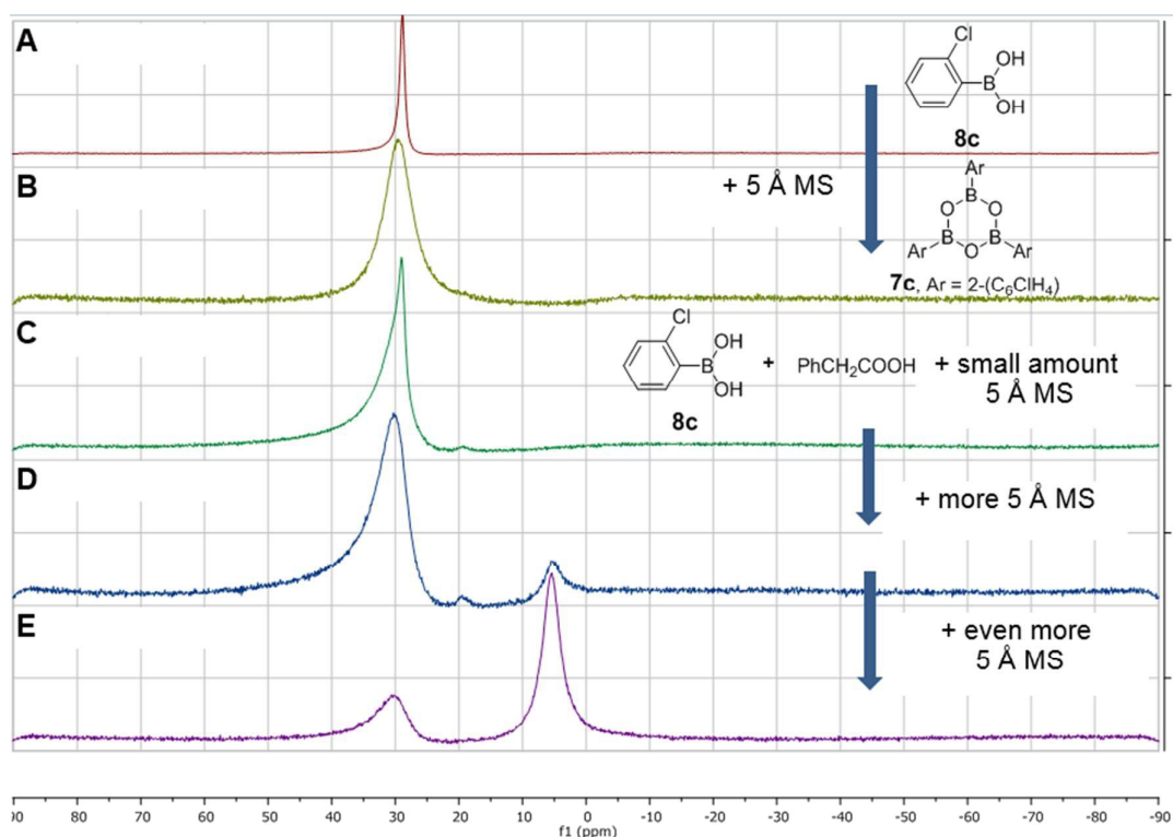
Figure 7. 11 B NMR spectra showing interactions between 2-chlorophenylboronic acid 8c , phenylacetic acid and 5 Å MS. A: 2-chlorophenylboronic acid; B: addition of 5 Å MS to (A), leading to boroxine formation; C: addition of a tiny amount of 5 Å MS to a mixture of boronic and carboxylic acid; D: addition of more 5 Å MS; E: addition of even more 5 Å MS.
