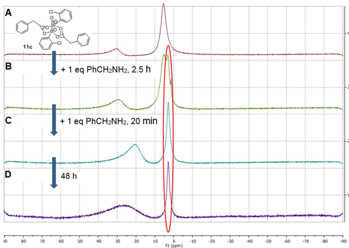
Figure 8. ^{11}\text{B} NMRs of A): mixture of 2-chlorophenylboronic acid 8c and phenylacetic acid in the presence of 5 Å MS resulting in equilibrium between B-O-B dicarboxylate 11c ( \delta 5 ppm) and boronic species 7c ( \delta 30 ppm); B): addition of 1 equivalent (per “ate”-complex 11c ) of benzylamine, 2.5 h, showing formation of a new complex 12 ; C): Addition of 2 nd equivalent of benzylamine, 20 min; D): Same mixture over 48 h.
