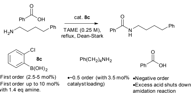
Scheme 12. Preliminary kinetics studies on a boronic acid catalyzed amidation reaction.
