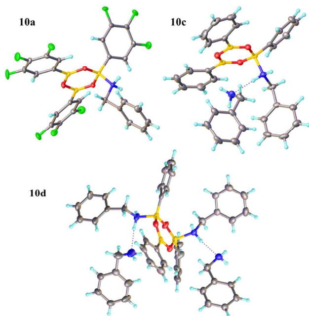
Figure 5. X-ray structures of 3,4,5-trifluorophenylboroxine-benzylamine adduct 10a and phenylboronic acid derived boroxine-amine adducts 10c and 10d .
