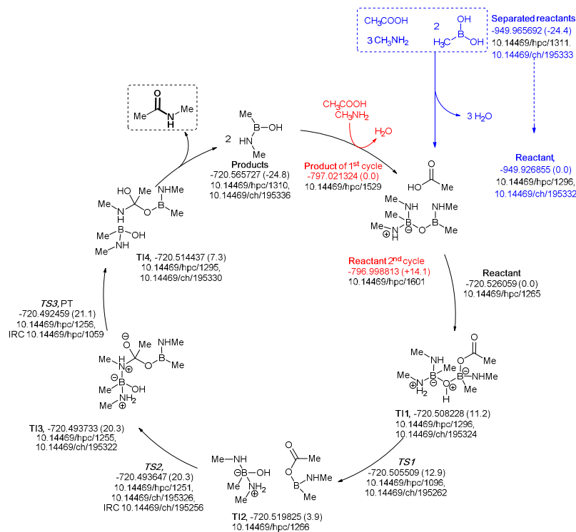
Figure 11 Catalytic cycle involving three amines (data 26 sub-collection DOI: 14469/hpc/1621; the labels have the same meaning as in Fig. 9).
