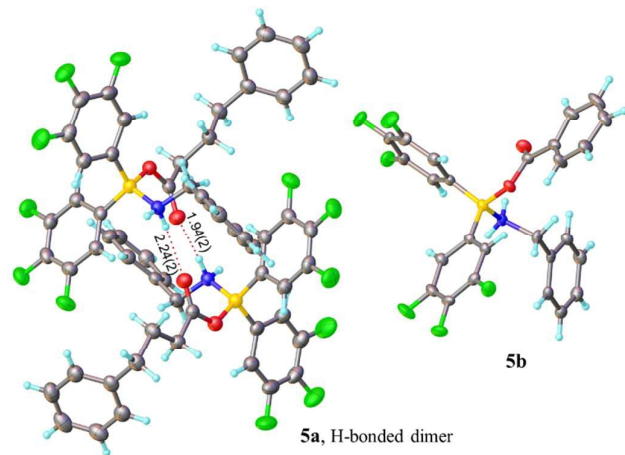
Figure 2. X-ray structures of amino-carboxylate borinic complexes 5a (showing a hydrogen-bonded dimer of two independent molecules) and 5b (disorder of phenyl ring is omitted for clarity). For 5c and 5d see ESI.
