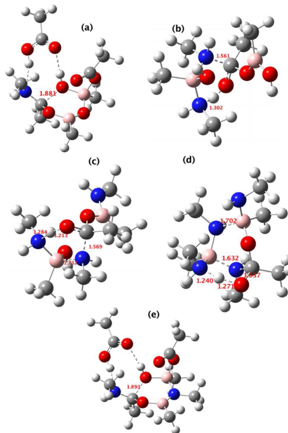
Figure 14. The computed structure for: a) TS3 shown in Fig. 9; b) TS3 shown in Fig. 10; c) TS3 shown in Fig. 11; d) TS1 shown in Fig. 12 and e) TS2 shown in Fig. 13. Indicated bond length are in Å. The activation free energies \Delta G_{298}^\ddagger for the five transition states are respectively 23.4, 25.2, 21.1, 25.4 and 23.2 kcal mol -1 .
