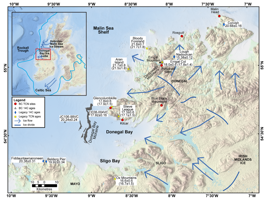
Figure 1. Location map of Donegal and parts of Sligo and Mayo with terrestrial legacy ages (TCN and ^{14}\text{C} ), BRITICE-CHRONO ^{14}\text{C} ages for the Donegal Bay Moraine, with core numbers, and sites of new TCN ages reported in this paper. Only those legacy ages of relevance to deglaciation are shown. The first TCN age for each site was calculated using version 3.0 of the online exposure age calculator formerly known as the CRONUS-Earth online exposure age calculator with the LLPR; the age in parentheses was calculated using CRONUS-calc 2.0. Ages are mean values of two or more ages for each site except for Glencolumbkille, which is represented by a single age. Terrestrial ^{14}\text{C} ages are minimum ages for deglaciation. Ice divides and generalized ice flow directions are from Greenwood and Clark (2009a). Inset shows location of Donegal and the LGM limit of the BII.
