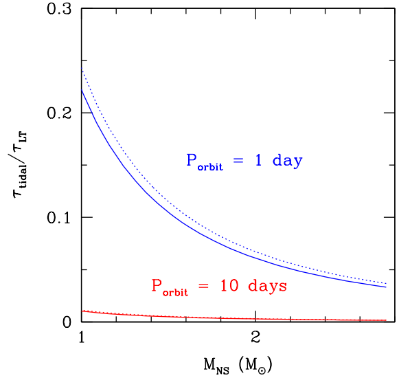
Figure 7. The ratio of the respective tidal to Lense-Thirring torques assuming a mass for the secondary star in the range of 18 (solid line) - 23 (dotted line) M_{\odot} (Motch et al. 2014) and an orbital period consistent with observations of supergiant HMXBs (i.e. of order days, e.g. Corbett & Krimm 2013). Whilst we have assumed B = 1 \times 10^{12} G, we note that the torque ratio decreases with decreasing field strength. Clearly the Lense-Thirring torque is expected to dominate the flow.
