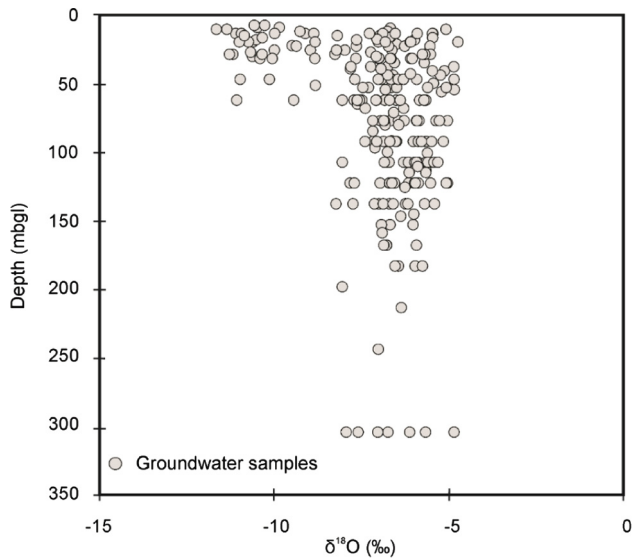
Fig. 4. \delta^{18}\text{O} variation with sampling depth for all groundwater samples within the study area. The distinction between samples taken generally above 80 mbgl are wider in range, which shows the multiple sources of recharge up to the depth of 80 m compared to samples below that depth.
