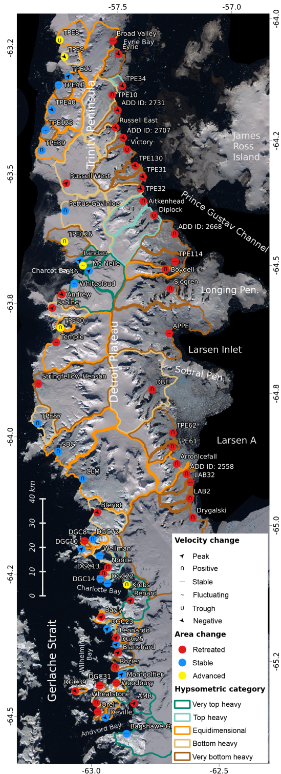
Figure 3. Categorizations of glaciers based on the temporal variations of area changes (dots) and flow velocities (symbols). Colors of catchment delineation indicate hypsometric categories according to Jiskoot et al. (2009). Background: Landsat LIMA Mosaic USGS, NASA, BAS, NSF.
