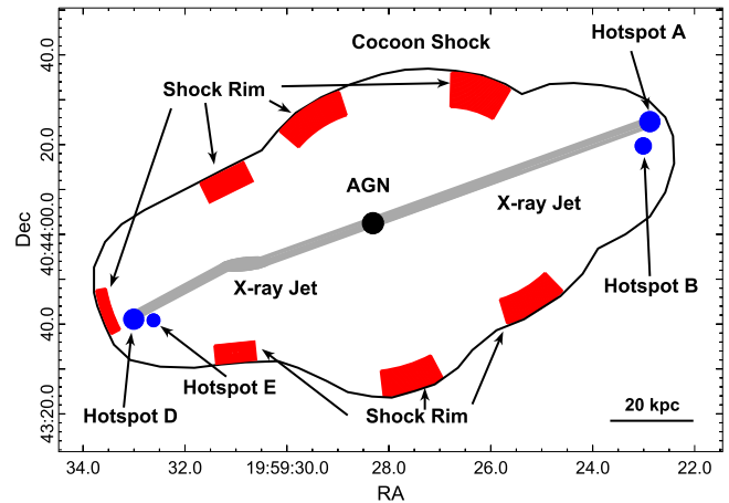
Figure 2. Schematic image of Cygnus A with key features (AGN, cocoon shock, hotspots, jets) labeled for ease of visibility. Several inner rims of the shock front that are visible in the original image are also highlighted.
