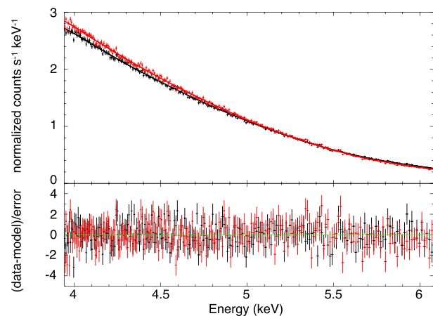
Figure 7. Chandra MEG \pm 1 count rate spectrum and the best-fitting continuum model. The black curve is MEG–1 and the red one is MEG+1.
