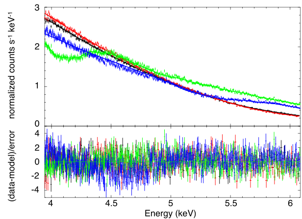
Figure A1. Chandra MEG±1 and HEG±1 count rate spectrum and the best-fitting continuum model. The black curve is MEG−1, the red one is MEG+1, the green one is HEG−1, and the blue one is HEG+1.
