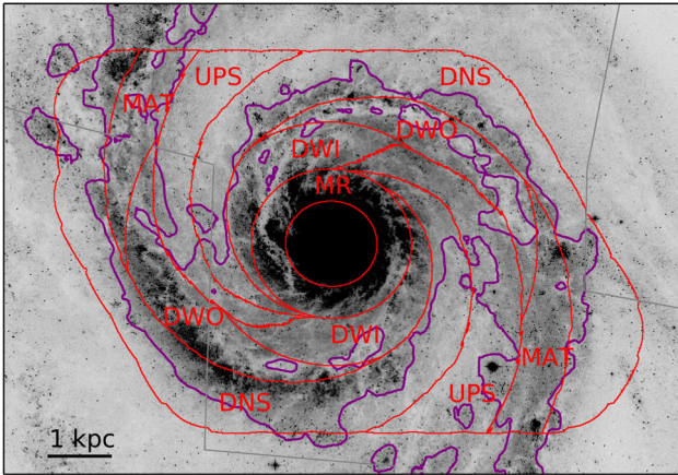
Figure 11. Dynamical regions as defined by C14 for the PAWS project (red contours), overplotted on the V-band frame and compared to the SA-IA division presented in Section 3 (purple contours).
