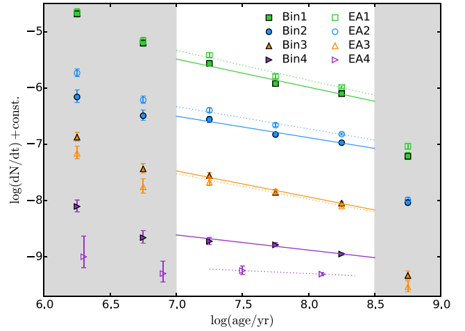
Figure 12. Age functions of the radial subsamples. Age bins are 0.5 dex wide, and the fit was performed only for points in the range \log(\text{age}) = 7-8.5 . In the case of EA4, the clusters in that age range have been divided into only two bins due to low-number statistics. Grey shaded regions mark the age ranges excluded from the fit. Fit results are given in Table 7.
