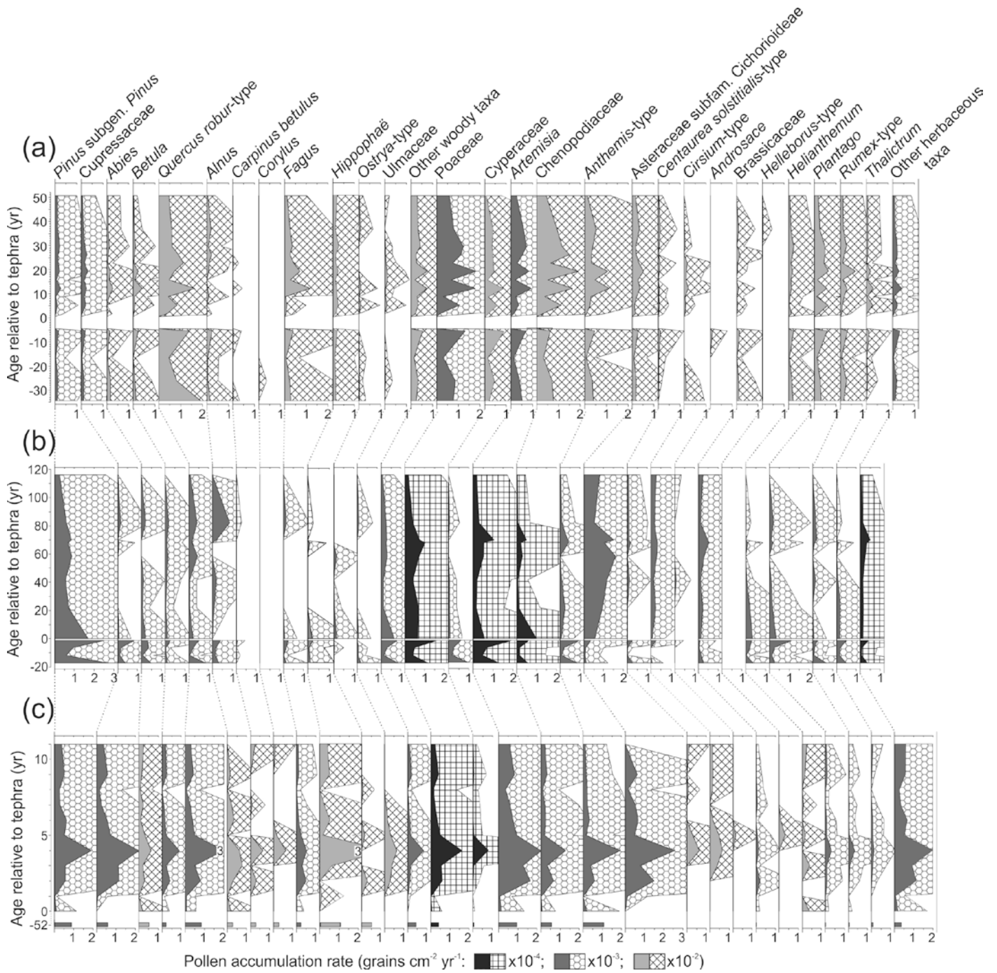
Figure 4: Pollen diagrams spanning tephra layers deposited when cold steppe prevailed
