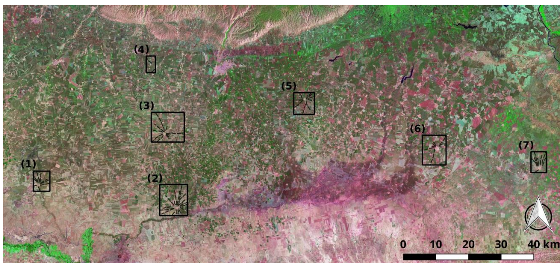
Figure 6. Sample areas representing the hinterlands of (1) Tell Beydar; (2) Tell Brak, (3) Tell Arbid, (4) Tell Mozan, (5) Tell Leilan, (6) Tell Hamoukar, and (7) Tell al-Hawa. The base map is a True-color Landsat mosaic imagery from the USGS.
