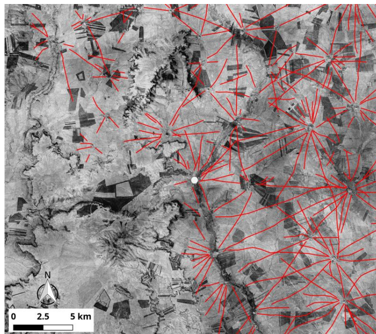
Figure 3. CORONA (DS1105-1025DA063; Nov 5, 1968) historical satellite imagery is an excellent source for mapping hollow ways with high precision. The basaltic landscape to the west of Tell Beydar (represented by the white dot at the center) does not contain evidence of movement, which may indicate differential route formation conditions or selective choices about movement.
