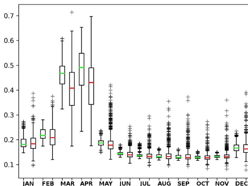
Figure 10. Monthly whisker-box plots of NDVI values of hollow ways (green) and the index values of randomly selected points from the whole scene (red). It is clear that March and April have the highest index values, and in these months hollow ways—on the average—are more separated spectrally than the background in comparison to other months. Nevertheless, more hollow ways are visible to the naked eye in May, making this a better month for mapping purposes.
