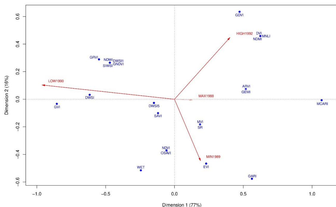
Figure 12. The Correspondence Analysis (CA) of significant indices from May.
