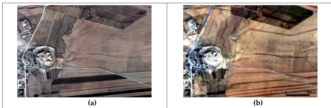
Figure 13. (a) Very High Resolution WorldView-3 satellite imagery (06 January 2017) still contain detailed evidence of hollow ways despite the impact of modern land-use practices on archaeological landscapes. (b) Sentinel-2 (24 February 2017) might have coarser resolution in comparison to WorldView-3, but with European Space Agency’s open-access policy, the system is a prime choice. The hollow ways still appear in great clarity on Sentinel2 Earth Observation satellites.
