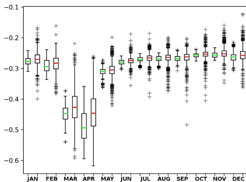
Figure 11. Monthly whisker-box plots of NDWI values. As in the case of NDVI, March and April have the highest spectral separation (green: hollow ways; red: background), but the November dataset is the most suitable for mapping due to the hollow ways being more visible to the naked eye.
