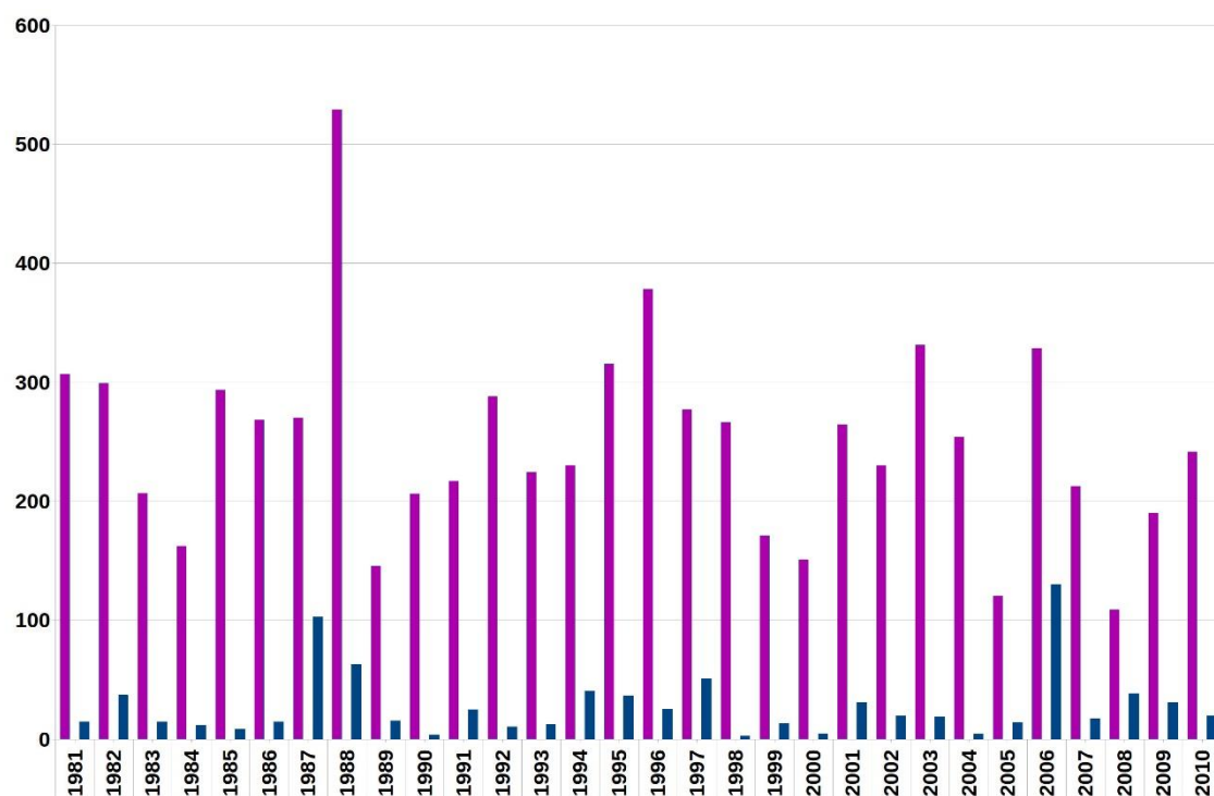
Figure 7. Averaged precipitation from all sample areas. Purple bars indicate accumulated precipitation values for May and blue bars for November. The wettest spring accumulation (by the end of May) was in 1988 and the wettest fall accumulation 2006 (by the end of November). The driest May accumulation was in 2008 and the driest November accumulation 1998. Other values range in between these years without an apparent trend.
