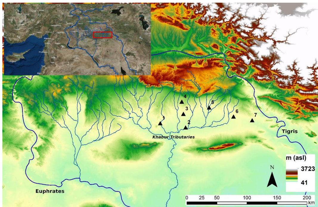
Figure 1. Upper Mesopotamia falls within the modern-day boundaries of Turkey, Syria, and Iraq. The study focuses on a selected portion of eastern Upper Mesopotamia (roughly depicted in the red bounding box), where the Khabur tributaries run between major Early Bronze Age settlements, such as: (1) Tell Beydar, (2) Tell Brak, (3) Tell Arbid, (4) Tell Mozan, (5) Tell Leilan, (6) Tell Hamoukar, and (7) Tell al-Hawa. The underlying Digital Elevation Model (DEM) is from the Shuttle Radar Topographic Mission (SRTM).
