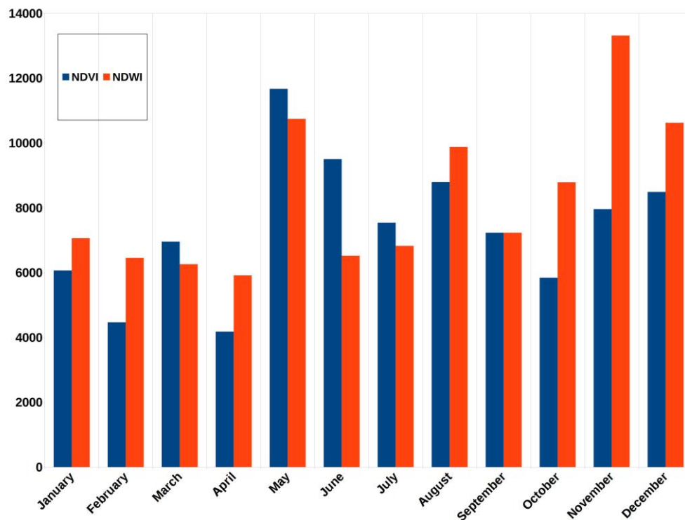
Figure 5. The total length of digitized hollow ways is represented in the y-axis (in meters). The variation between months can be attributed to differential vegetation growth and changes in soil moisture. For this sample, the May average detected the greatest proportion of the full extents of hollow ways for NDVI (11,672 m). For NDWI the November average maximized the documentation of hollow ways (13,317 m).
