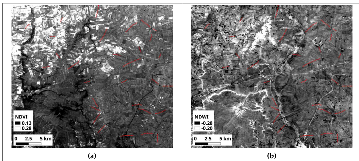
Figure 4. 30 sample hollow ways with variable lengths superimposed on (a) averaged Normalized Difference Vegetation Index (NDVI) values for May (2014–2017) and (b) averaged Normalized Difference Water Index (NDWI) values for November (2014–2017).
