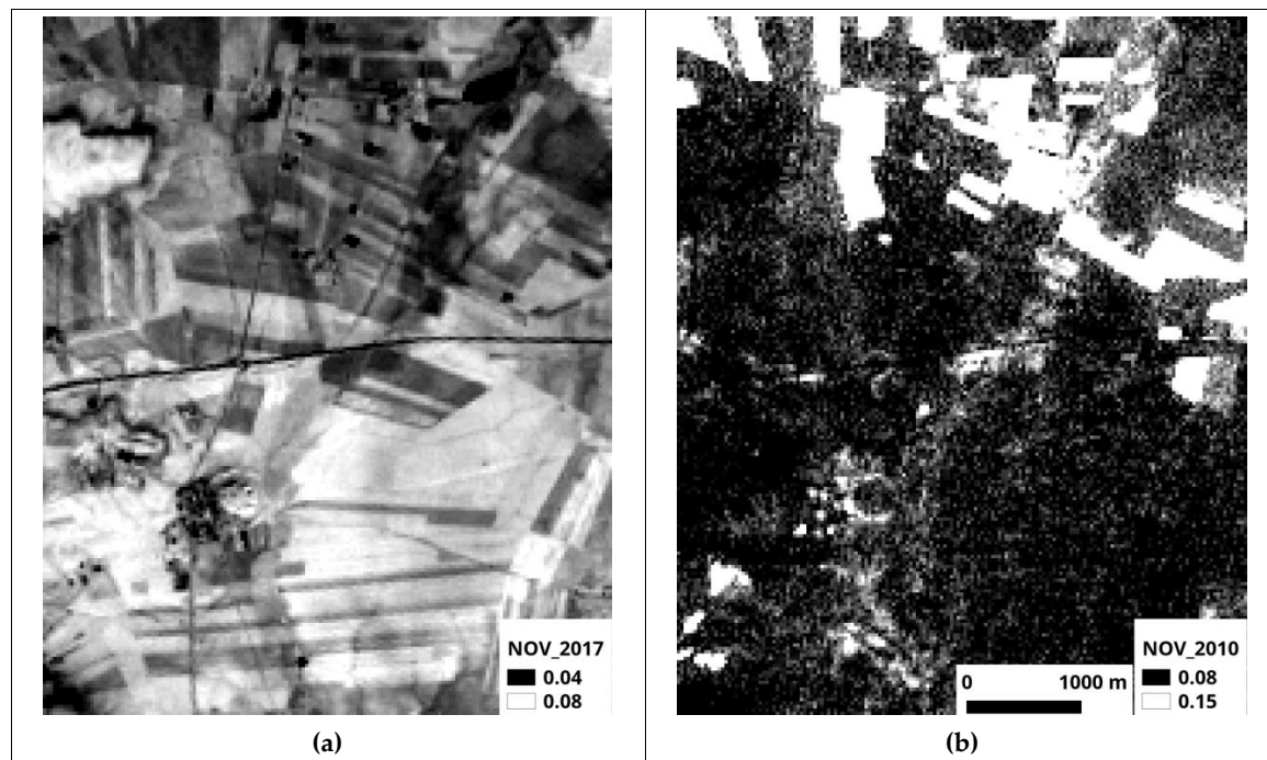
Figure 8. (a) NDVI values calculated from Landsat 8 for the area around Tell Beydar in November (2017) are high quality and ready for further statistical analysis; (b) Landsat 7 produces a lower-quality NDVI November dataset (2010) for the same area. Both datasets are displayed with the same rendering parameters.
