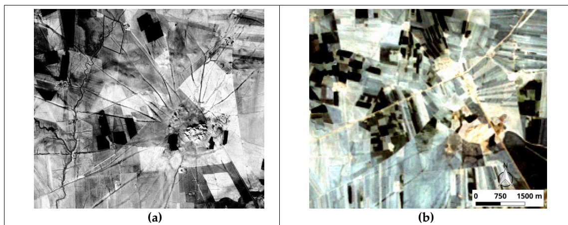
Figure 2. (a) Hollow ways radiating from Tell Brak (#2 on Figure 1) are clearly visible in CORONA imagery (DS1102-1025DA013, CORONA KH-4B; December 1967); (b) Landsat TM true color imagery (LT51710351990149RSA04; Landsat 5; May 1990) can also capture hollow ways, albeit to a lesser extent due to Landsat's lower spatial resolution, but also because of the impact of the mechanized land-use practices after the 1980s on cultural material.
