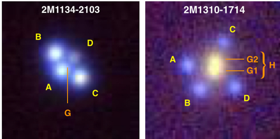
Figure 1. PS1 image extracts ( 15 \times 15 \text{ arcsec}^2 ) of 2M1134–2103 (left) and 2M1310–1714 (right), constructed from gri data. Labels identify the quasar images A–D and the lensing galaxies. For 2M1134–2103, the lens is not seen in this image; for 2M1310–1714 we show schematically the two compact components (G1, G2) and one extended component (H) used to model the lens.
