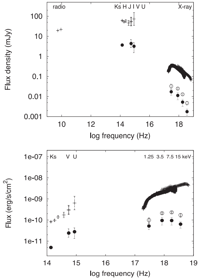
Figure 3. Top panel: broad-band SED spanning radio with ATCA (Corbel et al. 2013b), Ks band with ISAAC, H , I , J , V bands with SMARTS (Buxton et al. 2012) and V , U bands with XMM-Newton OM and X-rays with XMM-Newton and RXTE . The XMM-Newton , RXTE , ISAAC and OM data are simultaneous, while the other band data are closest to these observations. The spectrum of the QPO is shown with filled circles (QPOs around 0.08 Hz) and empty circles (QPOs at 0.16 Hz) in the bands as indicated in the bottom panel. Bottom panel: the QPO spectrum in flux units in the bands 0.5–2 keV, 2–5 keV, 5–10 keV, and 10–30 keV, where the mid-point of X-ray bands is shown along with the mean spectrum. The errors on the OIR QPO and mean spectrum are dominated by dereddening uncertainty.
