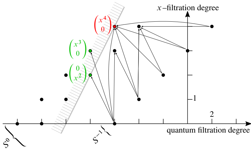
Figure 2: The filtered complex S in cohomological grading -1 and 0 , special case n = 5 , as a complex of complex vector spaces, ie forgetting the x -action. Dots represent copies of \mathbb{C} and arrows nontrivial differentials. The colored dots indicate the support of representatives of [\psi] . Dots on or to the left of the gray line of slope 1 lie in \mathcal{G}_{1/2}^{-5}S .
