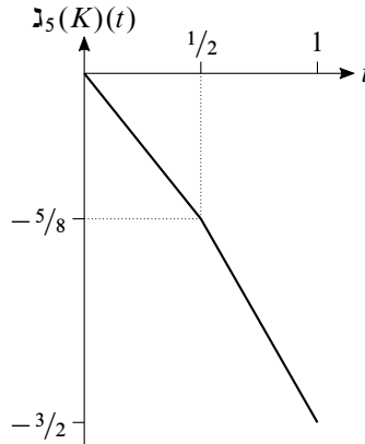
Figure 3: \mathfrak{J}_5(K) for K the P(2, -3, 7) pretzel knot
