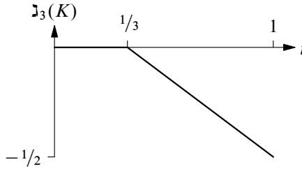
Figure 5: \mathfrak{J}_3(K) for K = P(7, -5, 4) \# P(-9, 7, -6)
