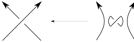
Figure 4: Adding two 1–handles, one on each side of a crossing
