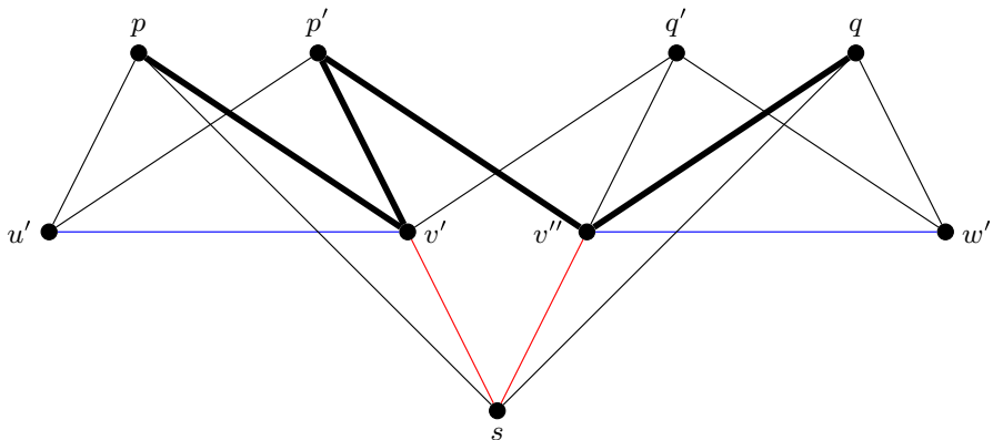
Fig. 8 An illustration of Case 2 of Claim 1 with the forbidden P_5 shown in bold. The red edges sv' and sv'' are present in both G and H . The blue edges u'v' and v''w' are present in H , but not G . The vertices p, p', q, q' are present in G , but not H , and the same holds for all of their incident edges. Note that the vertices p' and q' are not necessarily distinct. The edges pw' , p'w' , qu' and q'u' may or may not be present in G (Color figure online)
