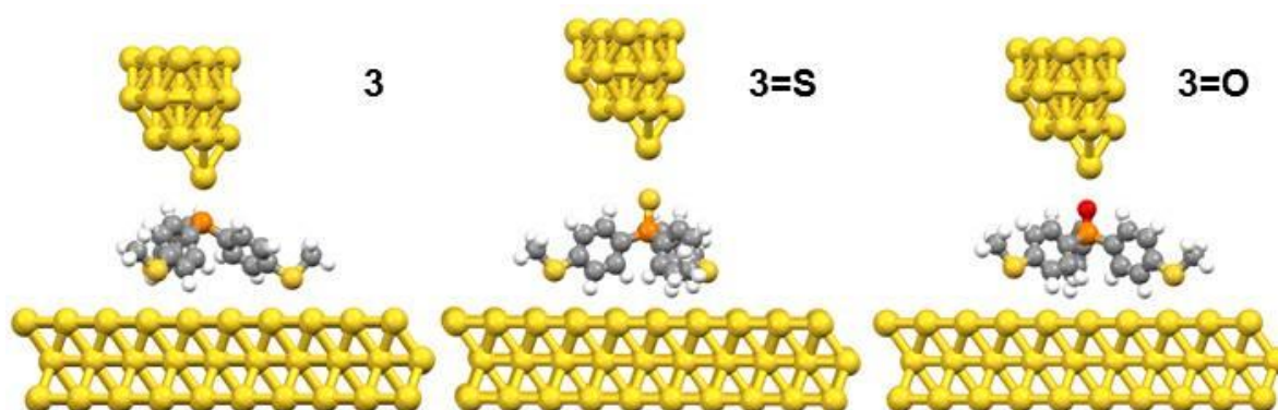
Figure 3. The relaxed geometries of all molecular junctions; where atoms are indicated by grey (carbon), white (hydrogen), yellow (sulfur), red (oxygen) and orange (Phosphorus).
