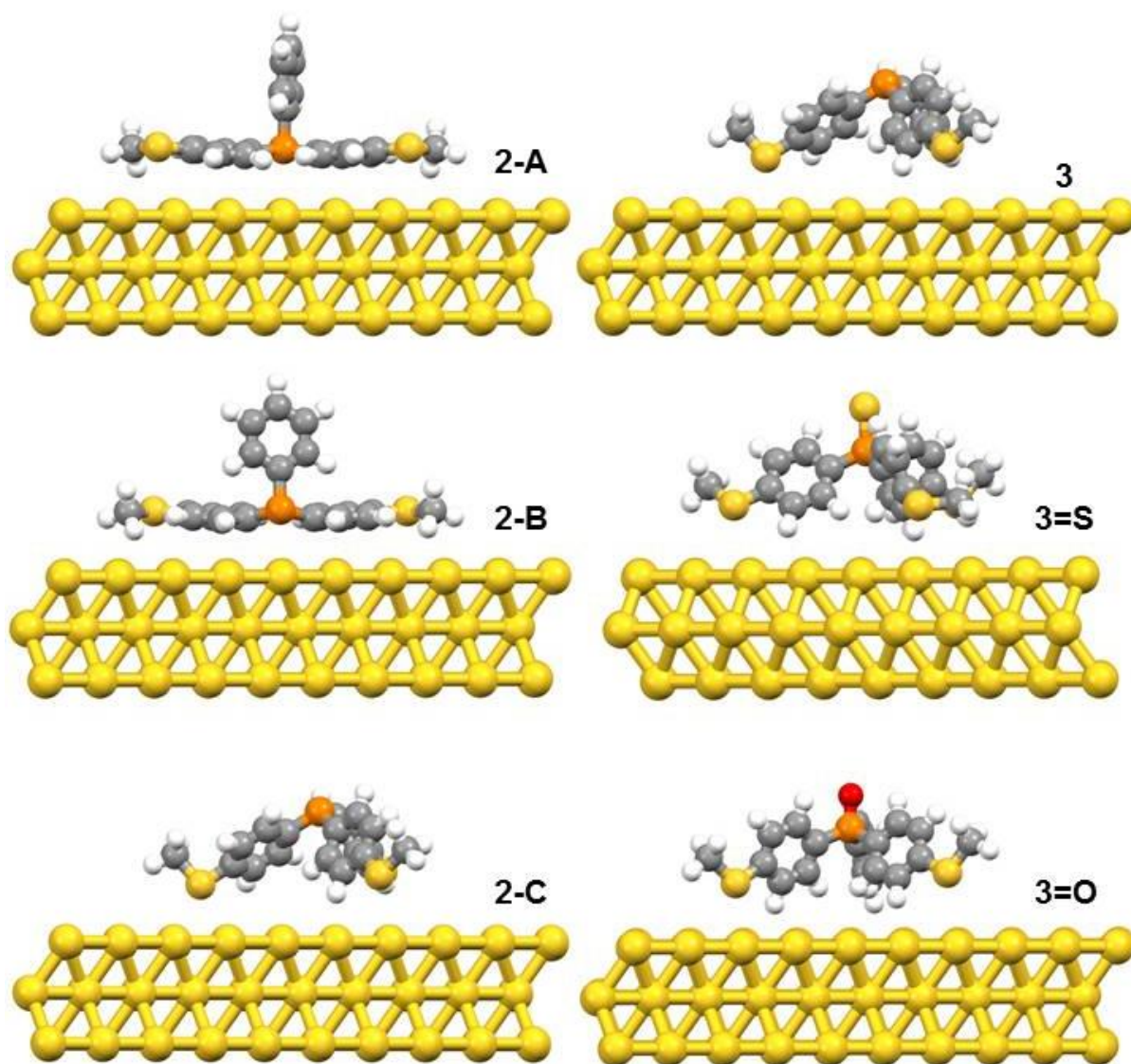
Figure 2. The relaxed geometries of all possible structures for 2 , 3 , 3=S and 3=O ; where atoms are indicated by grey (carbon), white (hydrogen), yellow (sulfur), red (oxygen) and orange (Phosphorus).
