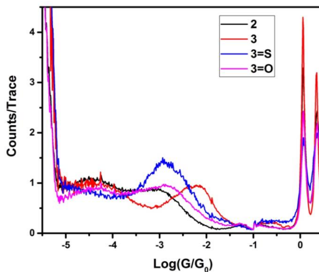
Figure 1. Conductance histograms for the compounds 2 , 3 , 3=S and 3=O .
