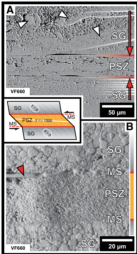
Figure 3. Close-up scanning electron microscopy images of Stages III and IV principal slip zone (PSZ) cross sections (same sample as in Fig. 2D, v = 1.4 \text{ m s}^{-1} , \delta = 90^\circ ). A: Back-scattered electron image showing relict (highlighted with white lines) and the last active (red lines) “mirror-like surfaces” (MSs); white arrows indicate the older, irregular, reworked MSs; red arrows indicate direction of migration of the PSZ boundaries during localization. SG—sintering gradient. B: Fore-scattered electron image of PSZ displaying oblique foliation, sharp grain-size transition at the boundaries, and MSs locally split and filled with epoxy during sample preparation (red arrow). Textures inside and outside the PSZ are clearly asymmetric with respect to MSs. In the inset, a schematic model of simple shear is compared to the microstructures. \gamma —angular strain.
