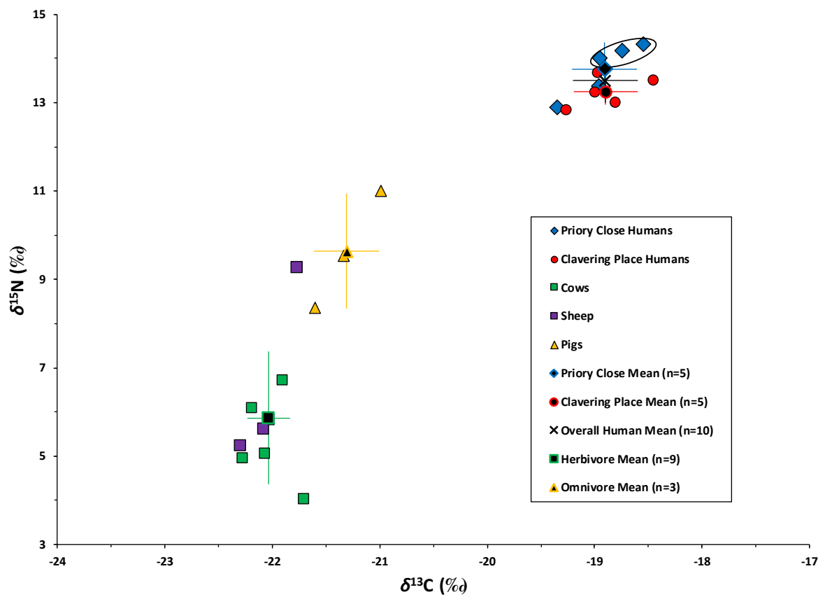
Figure 8. Individual and mean \delta^{13}\text{C} and \delta^{15}\text{N} values of individuals analyzed in this study. The individuals associated with DISH are circled. Means are shown with error bars of \pm 1 standard deviation.
