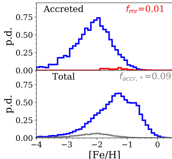
Figure 8. Similar to Fig. 4, but for satellite dwarfs with r_{mr}/r_{mp} < 0.65 : histograms of metallicity for stars that have been accreted (upper figure) and for the total stellar population (bottom figure).
