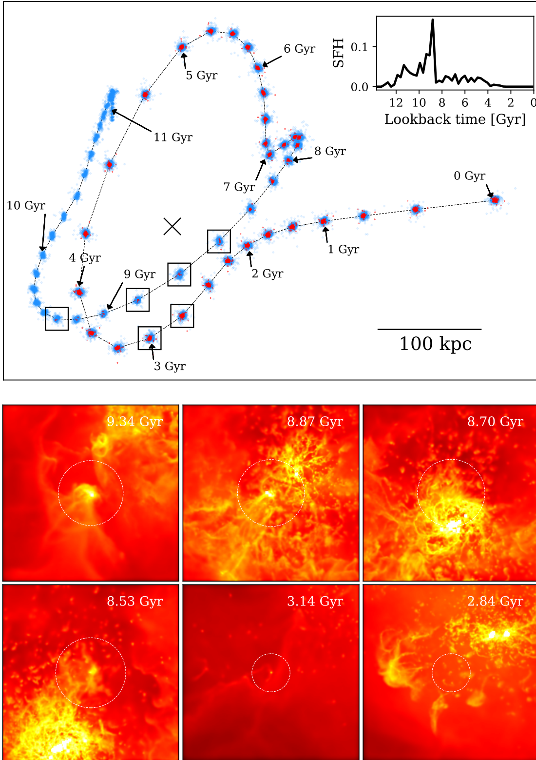
Figure 11. Top panel: The evolution of the satellite (labelled S-3) since its first stars formed just before a lookback time of 11 Gyr. The thin dotted line tracks the orbit of the satellite in the reference frame of the host halo. The black cross shows the position of the host halo. The squares mark important stages of the satellite's evolution. Between 9 and 8 Gyr in lookback time the satellite passes through the pericentre. At ~3 Gyr it encounters a larger, more massive, satellite. The inset at the top right displays the star formation history. The abrupt changes in the orbit between 8 and 6 Gyr, are caused by a fluctuation in the centre of potential of the host halo as it merges with a massive object. Bottom panel: the evolution of the gas distribution during the six stages of the satellite's evolution, as shown with squares in the upper figure. Yellow shows high density and black shows low density regions. The circle indicates the virial radius before infall (~9.5 Gyr) and the tidal radius thereafter. The images show a cube of 50 kpc on a side.
