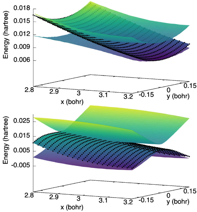
Fig. 7. First GI term of the TD PES, \epsilon_{GI1}(\mathbf{R}, t) , at t = 1000 au (surface with dotted lines), superimposed with the adiabatic PESs for both the weak- (upper) and strong-coupling regime (lower panel).
