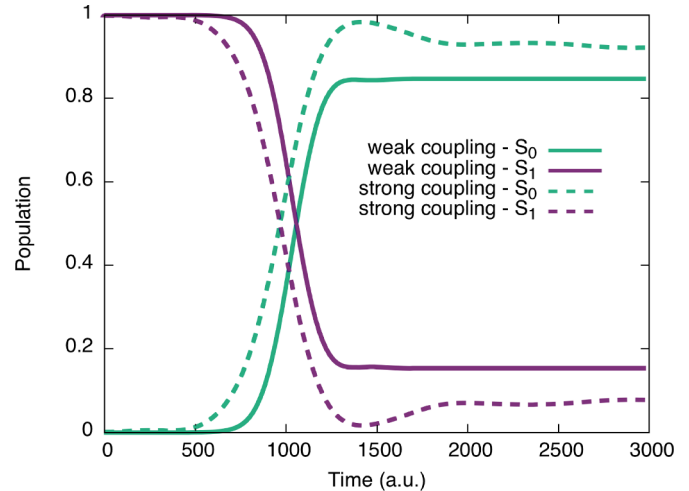
Fig. 3. Time trace of the adiabatic populations (green = S_0 , purple = S_1 ) during the nonadiabatic dynamics in the two different regimes considered: plain lines = weak coupling, dashed lines = strong coupling.
