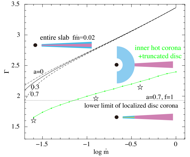
Figure 6. Same as Fig. 5b, but expected values of \Gamma_{\text{hot}} for slab geometry with L_{\text{diss,hot}} = 0.02L_{\text{Edd}} (i.e., f\dot{m} = 0.02 with the fraction of power dissipated in the corona, f ) are shown in black lines, together with the observed values of \Gamma_{\text{hot}} for Mrk 509, NGC 5548 and PG 1115 + 407 (open stars) and \Gamma_{\text{hot}} for truncated disc geometry with L_{\text{diss,hot}} = 0.02L_{\text{Edd}} (solid green). Albedo is assumed to be a = 0 (dash-dot), 0.3 (solid) and 0.7 (dash). Horizontal dotted straight lines represent the lower limit of \Gamma under an assumption of localized slab corona with maximal albedo, a = 0.7 and by assuming ‘passive disc’ underneath the corona, i.e., f = 1 .
