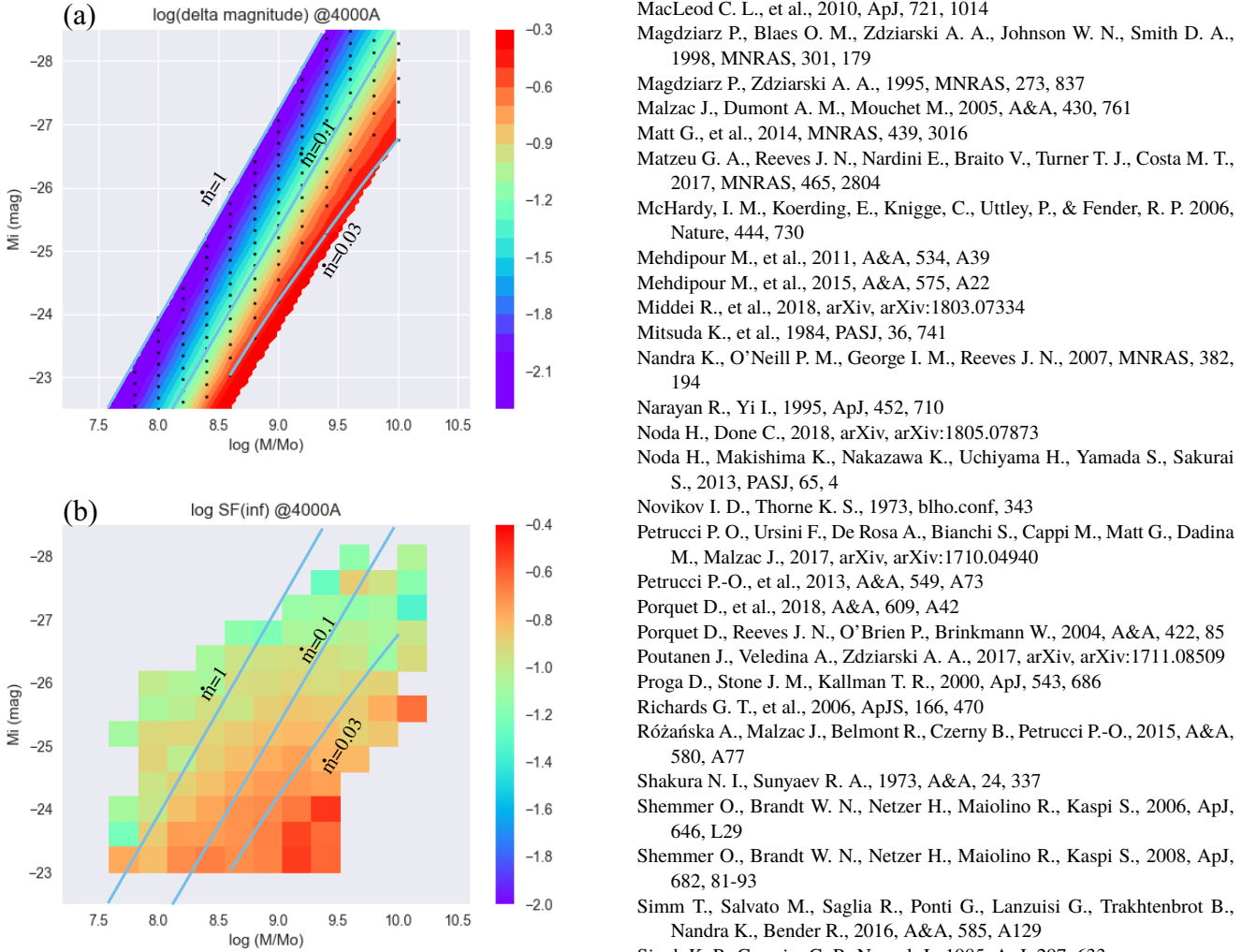
Figure 11. (a) Enlargement of Fig. 10b. Black dots represent the places which we calculate. (b) \log SF(\infty) at 4000\text{\AA} are plotted in space of M_i and \log M/M_\odot (Fig. 14 in MacLeod et al. 2010). These data points are given by C. MacLeod in private. Colour grid is the same between these two panels. Contours of constant \Delta mag in the top panel are overlaid on the bottom panel. Solid cyan lines show constant m of 0.03, 0.1 and 1.
