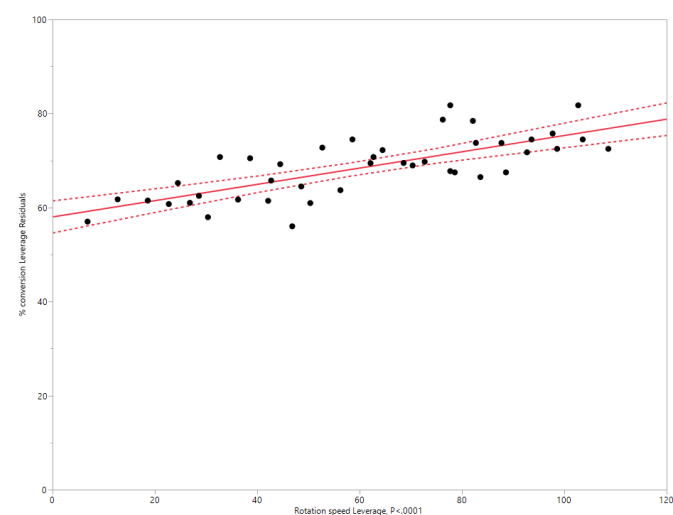
Figure 11. Modelling the HeRo process, demonstrating the relationship between rotation speed and % conversion estimated by ^1\text{H} NMR spectroscopy.
