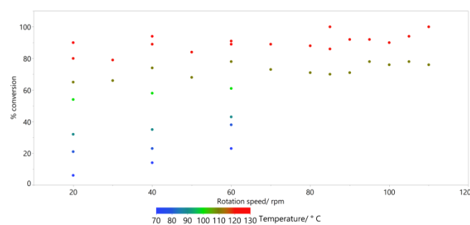
Figure 8. The effect of rotation speed on % conversion estimated by ^1\text{H} NMR spectroscopy for the HeRo process.
