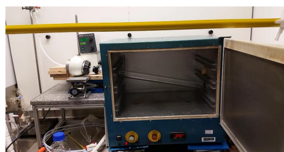
Figure 5. The HeRo reactor in situ , shown here with the oven door open to demonstrate the placement of the glass work-tube. The dropping funnel and tubing can be seen on the left, leading into the rotary drive which is connected to the work-tube. The material is collected in a flask situated behind the oven door.
