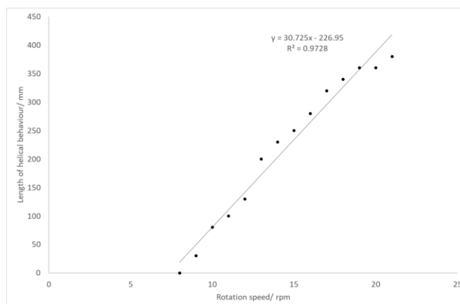
Figure 7. The effect of rotation speed on the length of the helix at 110 °C.
