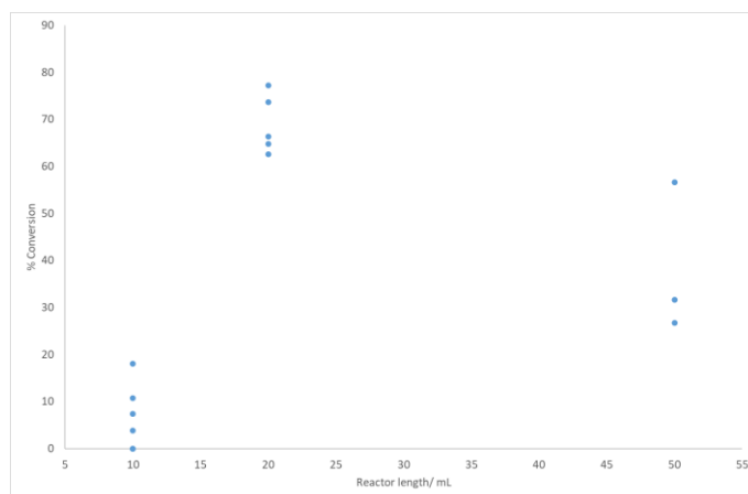
Figure 3. Reactor length plotted against % conversion to coumalic acid (assessed by 1 H NMR spectroscopy). Reactions were performed at 70 °C.
