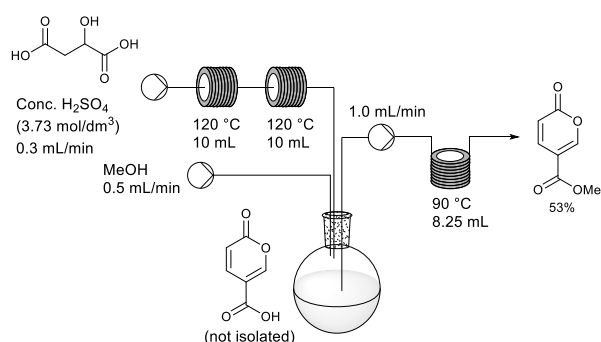
Scheme 8. Small-scale flow procedure for the synthesis of methyl coumalate.
