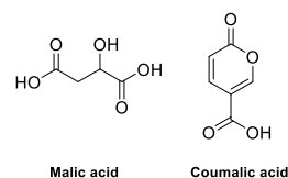
Figure 2. The biorenewable feedstock, malic acid, derived from glucose, and its dimerised condensation product coumalic acid.
