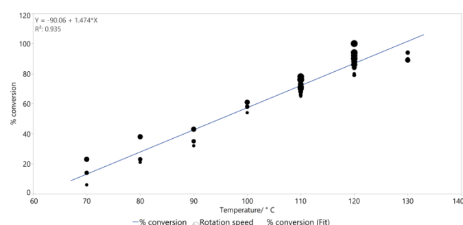
Figure 9. The linear relationship between temperature and % conversion estimated by ^1\text{H} NMR spectroscopy. Line of best fit: y = -90.1 + 1.47x and R^2 = 0.935 .
