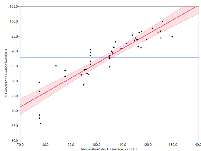
Figure 4. Impact of temperature on % conversion determined by ^1\text{H} NMR spectroscopy in the Vapourtec flow process.
