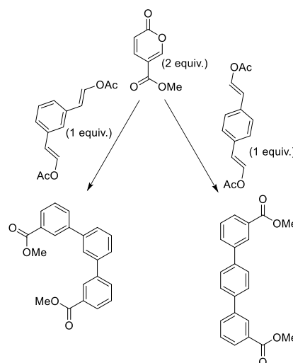
Scheme 10 –Potential Diels-Alder reaction between methyl coumalate and enol acetates.
