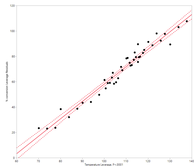
Figure 10. Modelling the HeRo process, plotting temperature against % conversion estimated by ^1\text{H} NMR spectroscopy.
