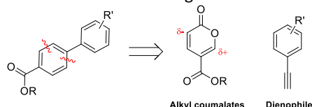
Figure 1. Retrosynthetic analysis, showing the substrates for the inverse electron
