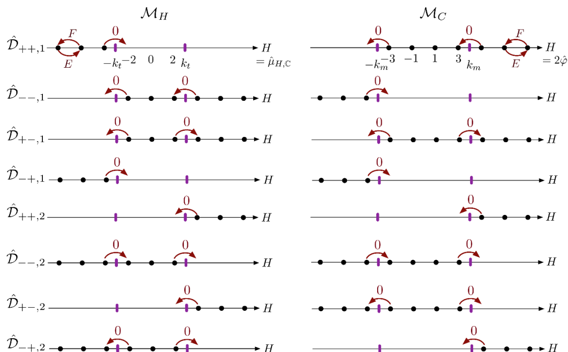
Figure 10. Modules for \hat{\mathcal{C}}[\mathcal{M}_H] and \hat{\mathcal{C}}[\mathcal{M}_C] corresponding to various exceptional Dirichlet boundary conditions in SQED with N = 2 hypermultiplets. To see the structure of standard (i.e. Verma) and costandard modules, we set t_{\mathbb{C}} = k_t \epsilon and (m_{1,\mathbb{C}}, m_{2,\mathbb{C}}) = \frac{1}{2} \epsilon (k_m, -k_m) for positive integers k_t, k_m \geq 1 . For each module, we depict the occupied weight spaces of the Cartan generator H (equal to \hat{X}_1 \hat{Y}_1 - \hat{X}_2 \hat{Y}_2 in \hat{\mathcal{C}}[\mathcal{M}_H] and \hat{\varphi} in \hat{\mathcal{C}}[\mathcal{M}_C] ). The \hat{\mathcal{C}}[\mathcal{M}_H] modules with k_t < 0 correspond to the same pictures modulo the substitution \hat{\mathcal{D}}_{\varepsilon_1, \varepsilon_2; 1} \leftrightarrow \hat{\mathcal{D}}_{-\varepsilon_2, -\varepsilon_1; 2} , while the \hat{\mathcal{C}}[\mathcal{M}_C] modules with k_m < 0 are described by replacing \hat{\mathcal{D}}_{\varepsilon_1, \varepsilon_2; 1} \leftrightarrow \hat{\mathcal{D}}_{-\varepsilon_1, -\varepsilon_2; 2} .
