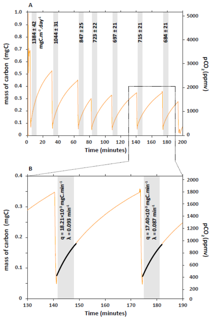
Figure 3: A: Series of carbon flux measurements for chamber H6 on 27/03/2017. CO 2 concentration (pCO 2 ) was converted into mass of carbon (mgC) following Eq. (4) and Eq. (5). Flux of CO 2 – the numbers associated to shaded boxes – are given in mgC.m -2 .day -1 . B: Close-up of how fluxes were calculated from the rate of carbon accumulation (parameter q) by fitting the exponential model described in Eq. (7) and (8) for 6 minutes (shaded box).
