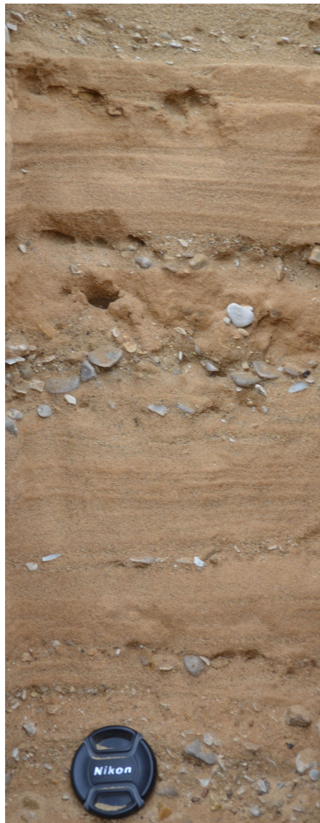
Figure 5. Details of LF1, showing horizontal to low angle planar cross-bedded sand with lags, separated by discontinuous lenses to beds of massive to horizontally bedded gravel.
