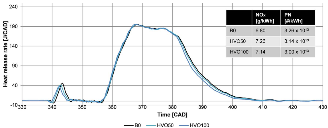
Fig. 15. HRR at point #8 – high speed and high load.
