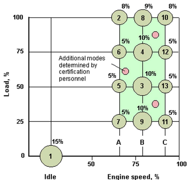
Fig. 6. European Stationary Cycle (ESC) [18].
