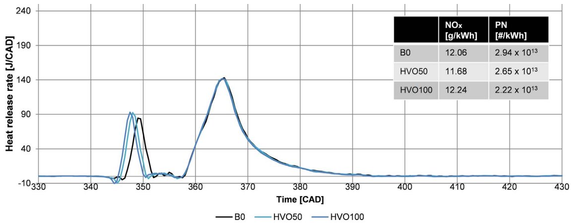
Fig. 14. HRR at point #7 – low speed and low load.
