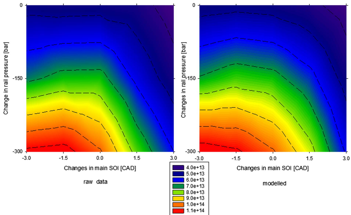
Fig. 21. Comparison of PN raw data and quadratic model at point #4.
