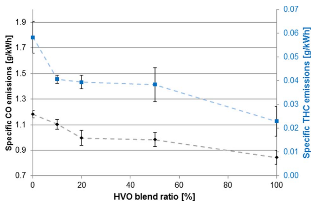
Fig. 11. Average specific CO (left) and THC emissions (right) with increasing HVO blend.
