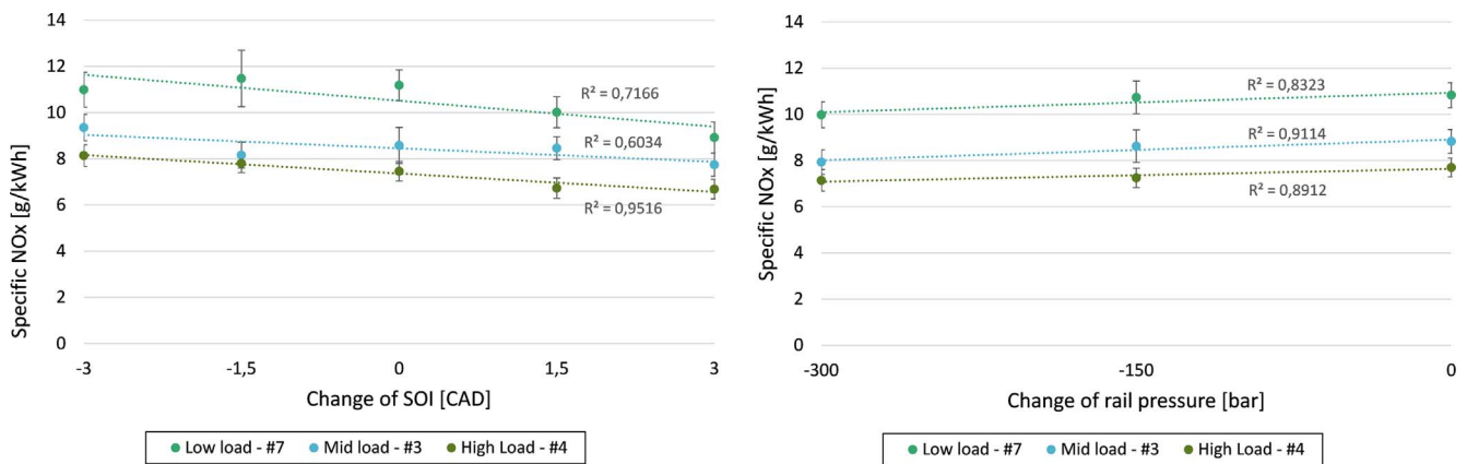
Fig. 18. NO x emissions as function of SOI and RP for all test points #3, #4 and #7.
