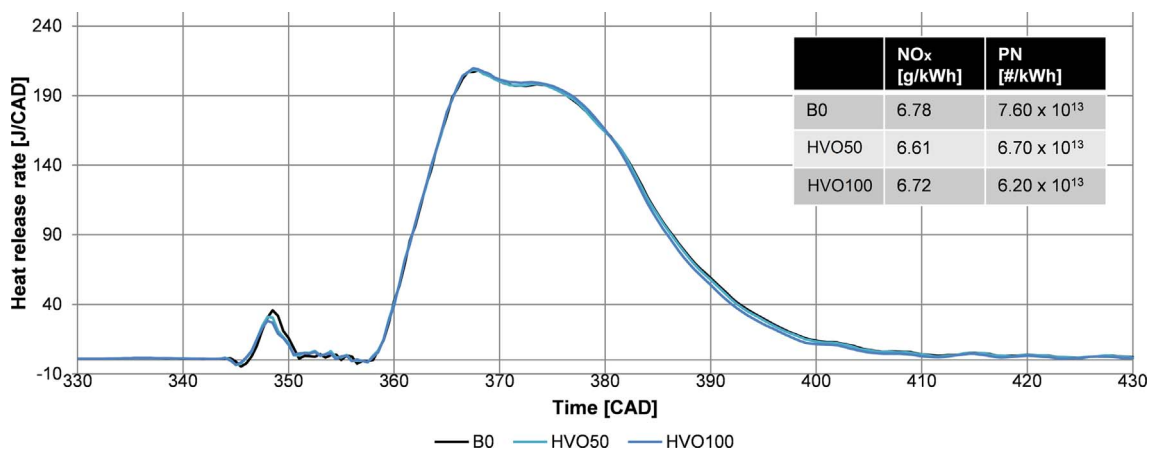
Fig. 12. HRR at point #2 – low speed and high load.
