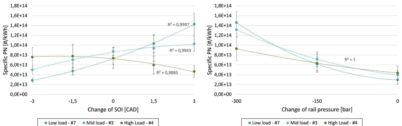
Fig. 19. PN emissions as function of SOI and RP.
