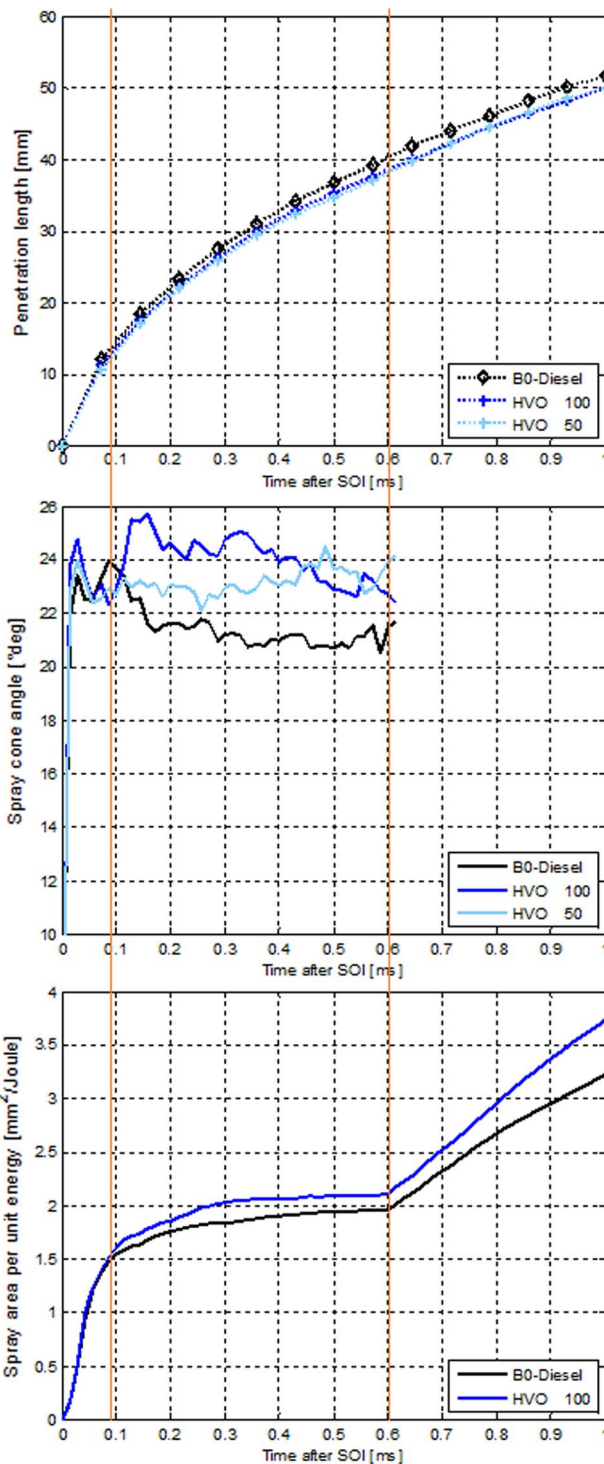
Fig. 7. Spray penetration (top), Spray angle (middle) and spray area per energy (bottom) for HVO and B0.
