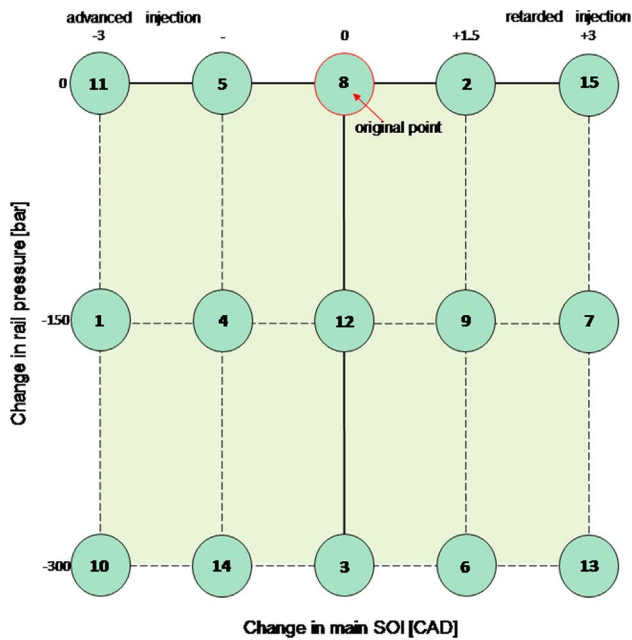
Fig. 17. Design of experiment for engine recalibration.
