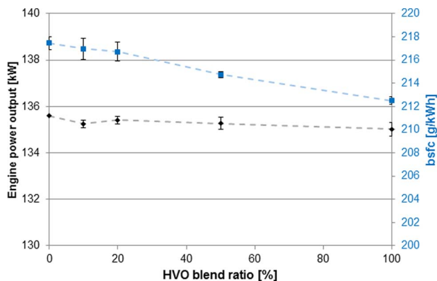
Fig. 8. Engine full power (left) and fuel consumption (right) with increasing HVO blend.
