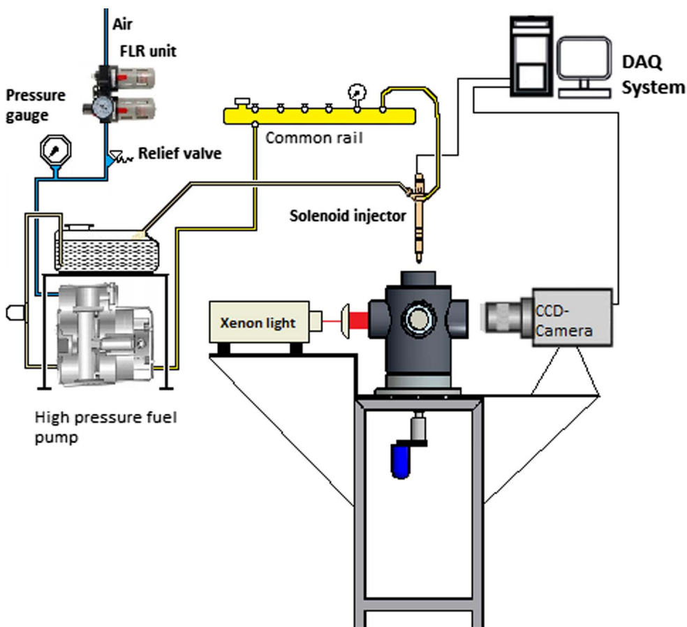
Fig. 2. Constant volume vessel set up.
