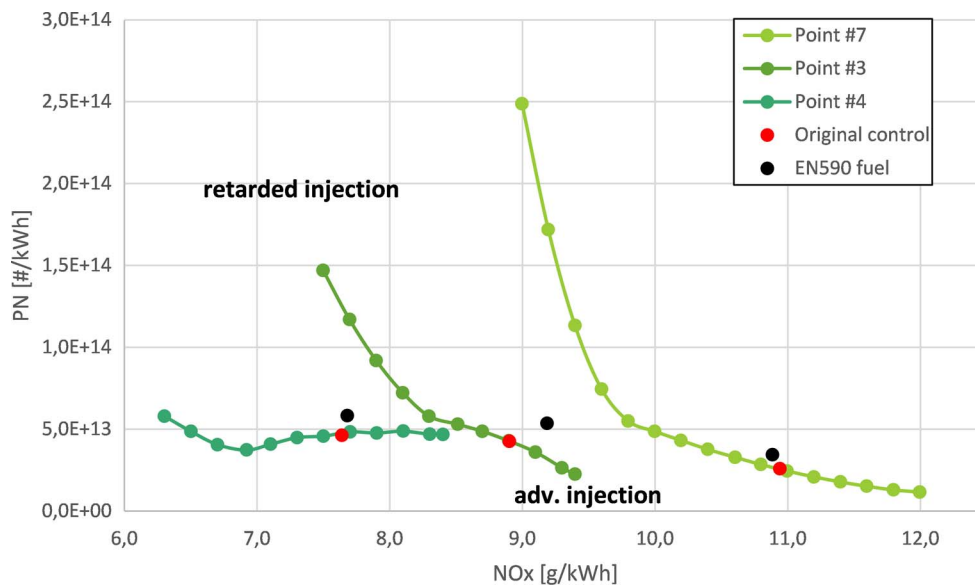
Fig. 22. \text{NO}_x -PN trade-off curves for point #7, #3 and #4 including the original control and benchmark.
