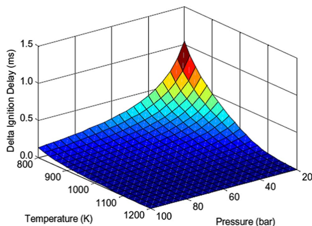
Fig. 13. Difference in ID as function of temperature and pressure [21].
