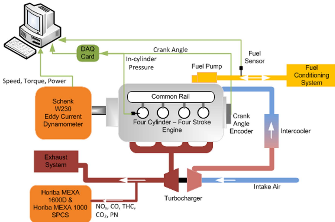
Fig. 5. Engine test setup.
