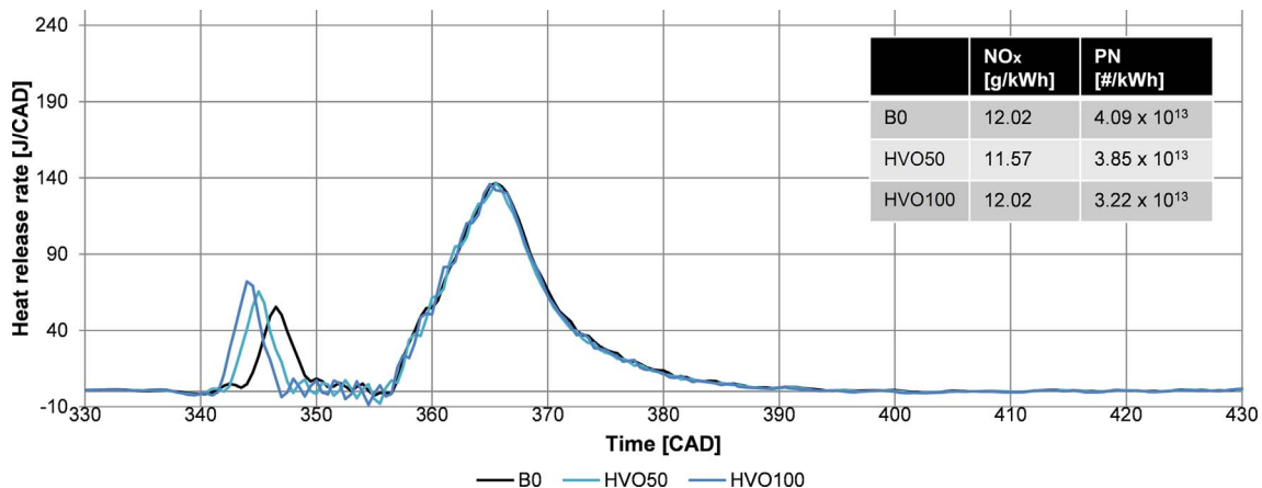
Fig. 16. HRR at point #9 – high speed and low load.
