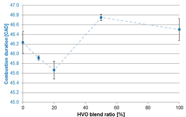
Fig. 10. Average combustion duration with increasing fuel blend.
