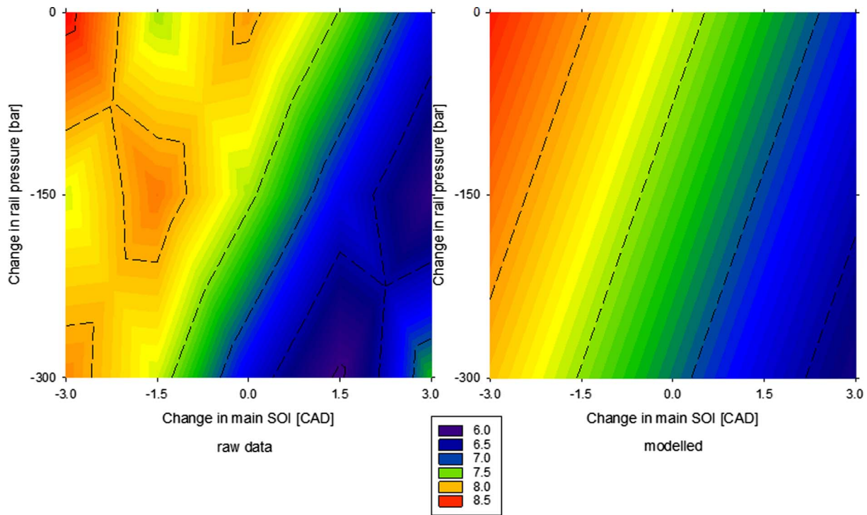
Fig. 20. Comparison of NO x raw data and linear model at point #4.
