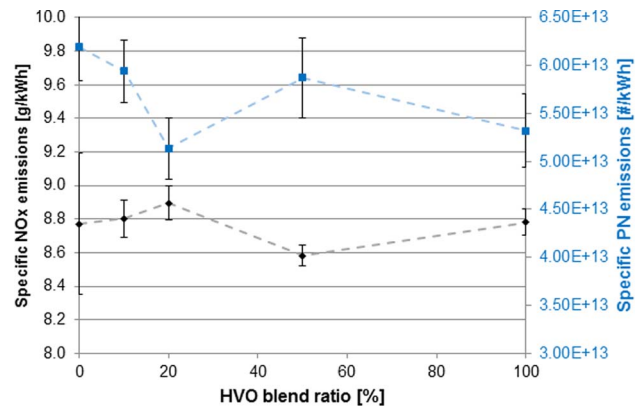
Fig. 9. Average specific NO x (left) and PN emissions (right) with increasing HVO blend.
