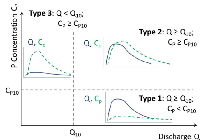
Fig. 3. Event classification method, according to the method of Haygarth et al. (2004) depending on the relative dynamics of the discharge (Q, blue solid line) and phosphorus concentration ( C_P , green dashed line). Q_{10} is the discharge exceeded 10% of the time; C_{P10} is the concentration of total phosphorus exceeded 10% of the time.
