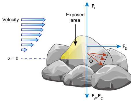
Figure 1. Components of the moment-balance model. Vectors F_L , F_D , F_W , and F_C are the lift, drag, grain weight, and cohesive forces, respectively. Red arrows show vectors of the grain center of mass and two contact points with downstream grains. Red dashed arrow shows resultant of these two vectors, which does not have to be in the downstream direction. Pivot angle ( \phi ) is the angle between this vector and vertical. Grain pivots around the black dashed line. Downstream velocity is zero at elevation z = 0 .
