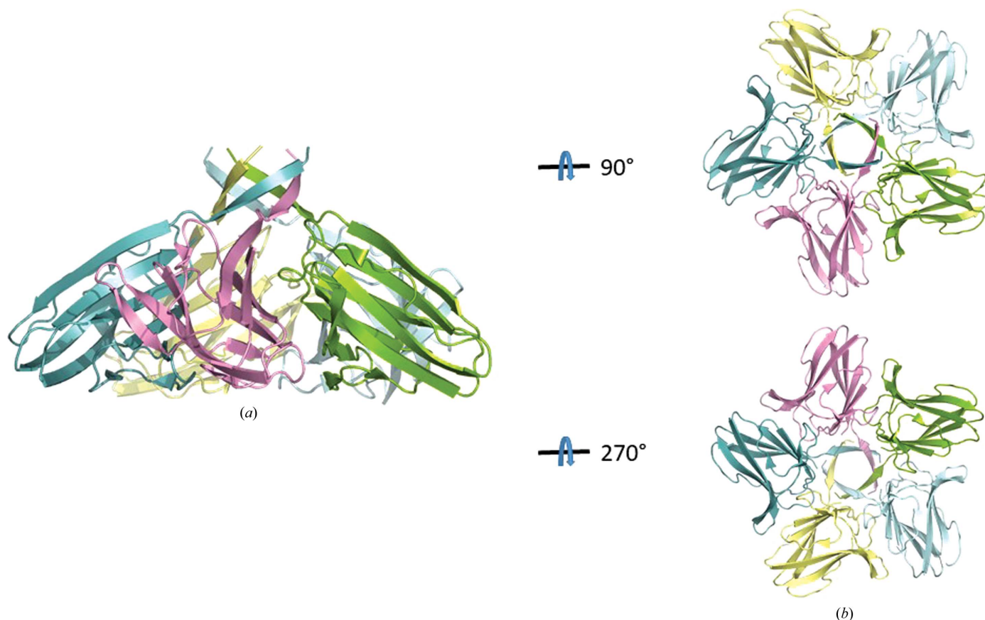
Figure 6 Ribbon diagram of the crystal structure of the YomS homopentamer. (a) Each polypeptide chain is depicted in a different colour. (b) Top view of the YomS pentamer and bottom view of the YomS pentamer.
