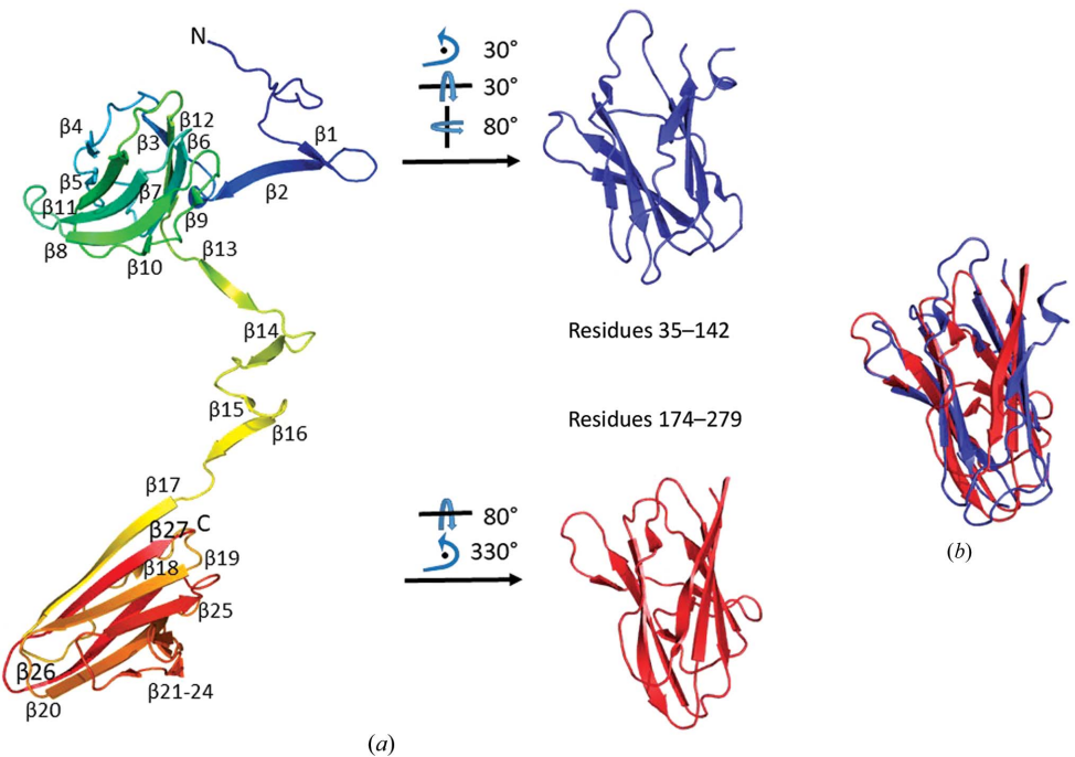
Figure 2 Ribbon diagram of the XepA crystal structure. (a) The monomeric unit, which is shown in rainbow colours from blue (N-terminus) to red (C-terminus) with annotation of all strands, reveals two \beta -sandwich folds that are connected by a linker region. The truncated N-terminal domain (blue) and C-terminal domains (red) are depicted in a reoriented position with the C^\alpha atoms used for least-squares superpositioning. (b) The \beta -sandwiches can be superimposed with an r.m.s.d. of 2.5 Å.
