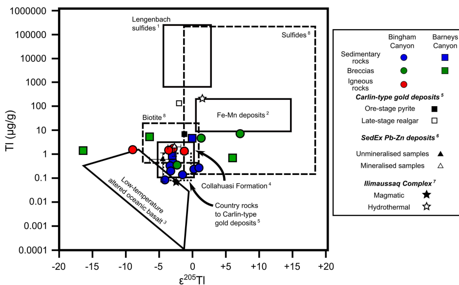
Figure 7. A plot of Tl concentration (µg/g) vs \epsilon^{205}\text{Tl} in samples from the Bingham Canyon district (this study) compared to literature data: 1 [56]; 2 [52,53]; 3 [39,40]; 4 [48]; 5 [54]; 6 [57]; 7 [55]; 8 [36].
