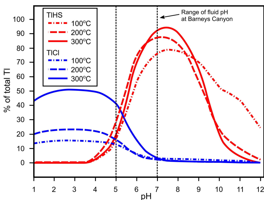
Figure 9. Modelled % of total Tl transported by \text{Cl}^- and \text{HS}^- anions in hydrothermal fluids plotted against fluid pH in reducing conditions at temperatures between 100–300 °C; modified after [63].
