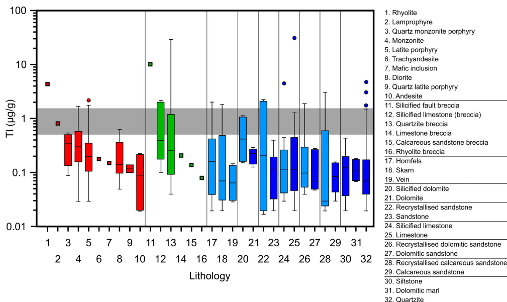
Figure 6. A box and whisker plot showing Tl abundance by lithology in all samples (n = 350) from the Bingham district, with samples grouped into broad lithological categories. “Boxes” denote the first and third quartile values, while the intermediate lines indicate median Tl contents; whiskers extend to the highest and lowest values, excluding outliers (circles), which are >1.5 times the inter-quartile range higher and lower than the third quartile and first quartile measurements, respectively; the solid squares indicate one measurement for a given lithology; colors as in Figures 4 and 5; pale blue color indicates recrystallized/silicified sedimentary lithologies. Note log-scale on y-axis; shaded box indicates range of estimates for Tl content of bulk continental crust [61].
