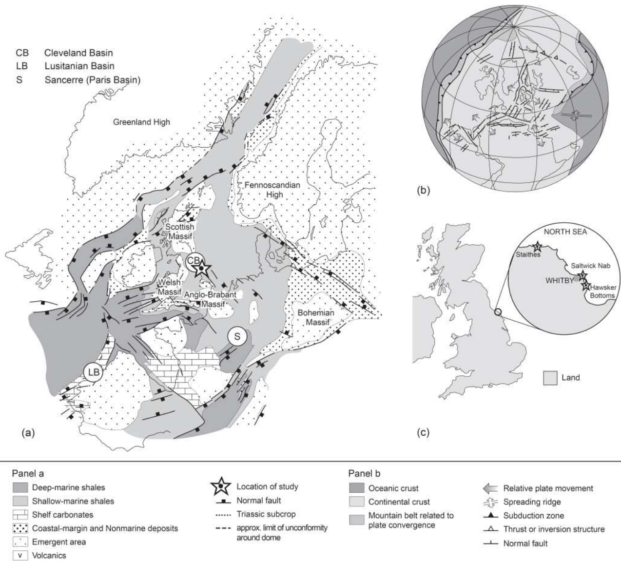
Figure 1: Early Jurassic palaeogeography of the studied area (a and b) modified after Coward et al. (2003) and Korte and Hesselbo (2011), with localities (stars) sampled (c). The star (a) marks the Yorkshire coastal outcrops in the Cleveland Basin (UK) situated in the Early Jurassic at 35–40°N.
