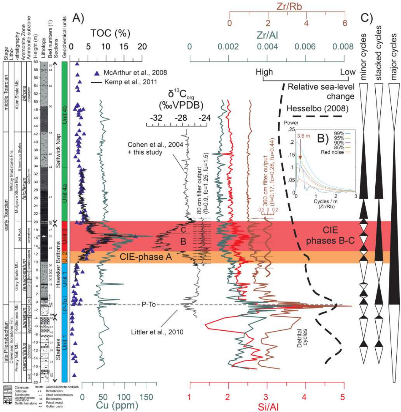
Figure 2. A) %TOC and Cu concentration, \delta^{13}\text{C}_{\text{org}} and trends in the ratio of siliciclastic elements (Zr/Al, Si/Al, Zr/Rb) compared to the relative sea-level curve of Hesselbo (2008). For the Toarcian carbon isotope excursion, we distinguish an interval corresponding to the onset of a progressive decrease in carbon isotopes (phase A of the CIE or Unit 2) and the remaining of the CIE (phases B-C) corresponds to geochemical Unit 3, whose base is defined by the first sharp, major drop in \delta^{13}\text{C}_{\text{org}} . A 80 cm filter output of \delta^{13}\text{C}_{\text{org}} data (Based on Kemp et al., 2005, 2011) is also presented along with an
