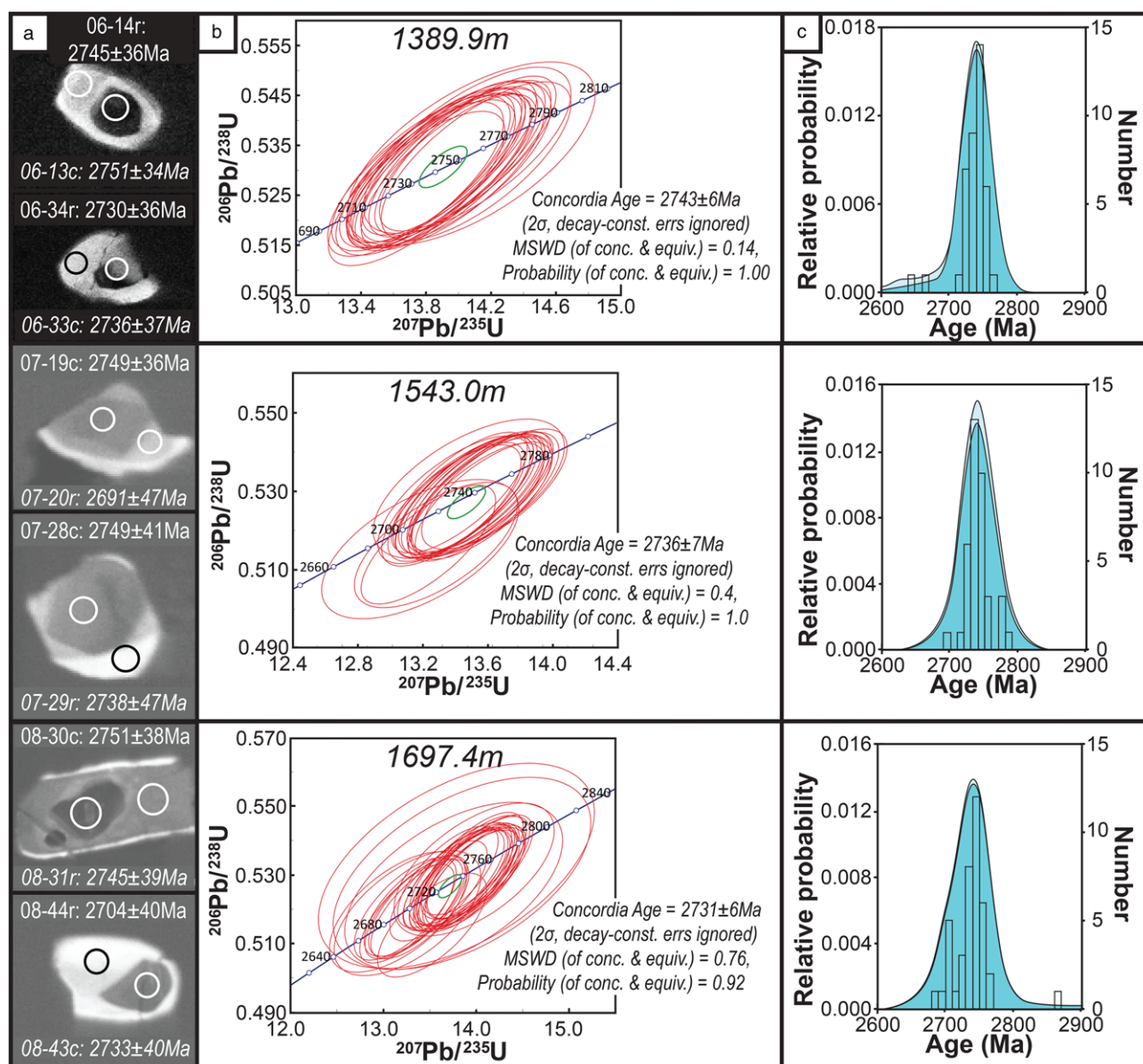
Fig. 11. U–Pb zircon geochronology from metatolalite samples at (a) 1389.9 m, (b) 1543.0 m and (c) 1697.4 m all from the 205/21a-7 well. (i) Representative CL images of zircons with 30 μm wide spot ages; (ii) U–Pb isotopic compositions of zircons displayed on Wetherill concordia diagrams, together with best estimates for zircon crystallization ages; all data-point error ellipses are 2σ; (iii) probability density plots of zircon ages from each of the samples.
