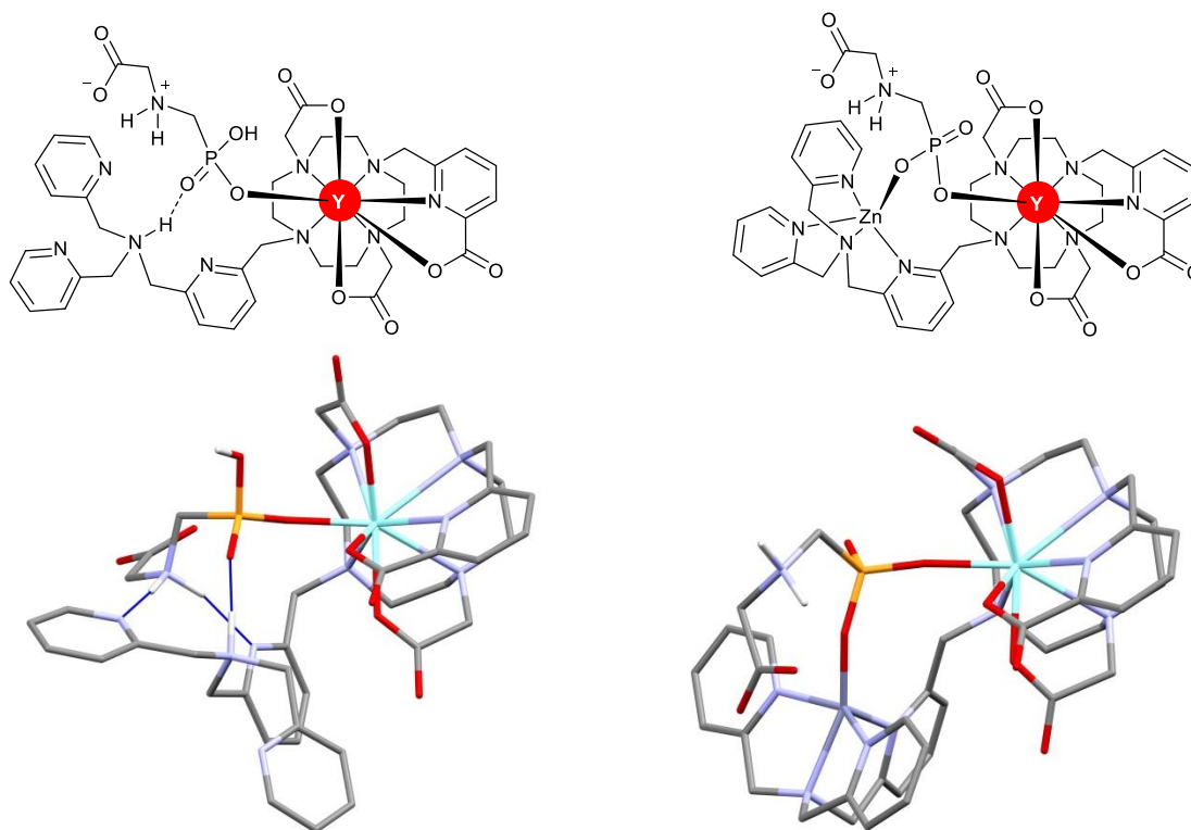
Figure 2 Optimised model geometries for [\text{HEuL}^1]\cdot\text{GlpH} and [\text{ZnEuL}^1]\cdot\text{GlpH} adducts, showing hydrogen bonding interactions. Hydrogen atoms bound to carbon are omitted for clarity, and Y is used as a surrogate for the Eu ion. The figures of optimised model geometries were generated using Mercury software. 31
