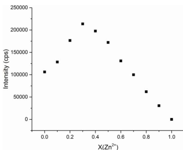
Figure 5 Job plot for [EuL 1 ] following the emission intensity change at 616 nm as a function of mole fraction ZnCl 2 ([EuL 1 ] 5 μM, 0.1 M HEPES, pH 7.40, 298 K, λ ex = 335 nm).
