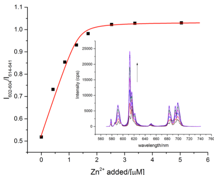
Figure 4 Variation of the emission intensity ratio and the overall emission spectrum of [EuL 1 ] ( inset ) with added ZnCl 2 ([EuL 1 ] 5 μM, 0.1 M HEPES, pH = 7.40, 298 K, λ ex = 335 nm), showing the large change in the form of the ΔJ = 1 manifold around 590 nm, consistent with a large change in the Eu coordination environment. The approximate binding affinity (log K = 7.5) was estimated using a simple 1:1 binding model.
