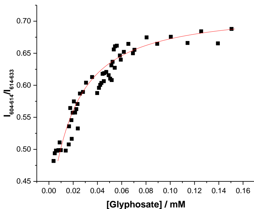
Figure 5 Variation of the Eu emission intensity ratio as a function of glyphosate concentration combining the ‘spiked grains’ data sets, showing the best fit ( line ), associated with an apparent log K value of 4.97.
