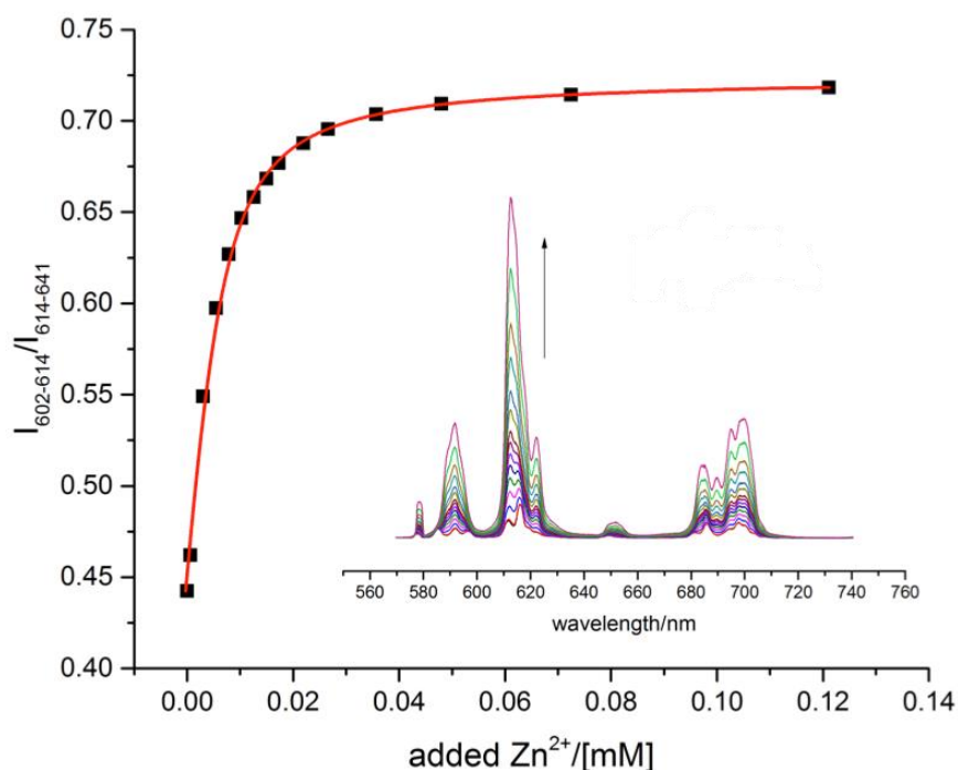
Figure 6 Variation of the europium emission spectrum ( inset ) and the intensity ratio for [EuL 2 ] with added ZnCl 2 , ([EuL 2 ] 8 μM, 0.1 M HEPES, pH = 7.40, 298 K, λ ex = 335 nm). The binding constant (log K = 5.6) was fitted using a 1:1 binding model.
