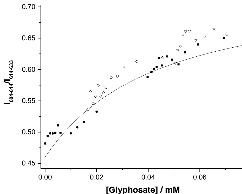
Figure 4 Comparison of the calibration curve ( line ) for [Eu.L 1 ](7 μM, 0.1 M NaCl, 0.1 M MES, 295 K, pH 5.9, \lambda_{\text{exc}} 365 nm) with the data points derived from addition of increasing glyphosate concentrations between 0-0.06 mM, to the ‘spiked grain’ extracts for different initial glyphosate concentrations: 60 μM (triangles), 30 μM (squares), 15 μM (diamonds), 7.5 μM (circles).
