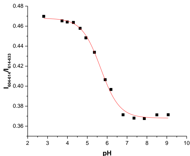
Figure 1 Variation of the europium emission intensity ratio (604-614 nm / 614-633 nm) with pH for [Eu.L 1 ] ([complex] = 7 \mu M, 0.1 M NaCl, 295 K, \lambda_{ex} 340 nm), showing the fit ( line ) to the experimental data points (Table 1). At higher pH (>11), bicarbonate may bind competitively to the Eu centre, displacing a coordinated pyridine donor.
