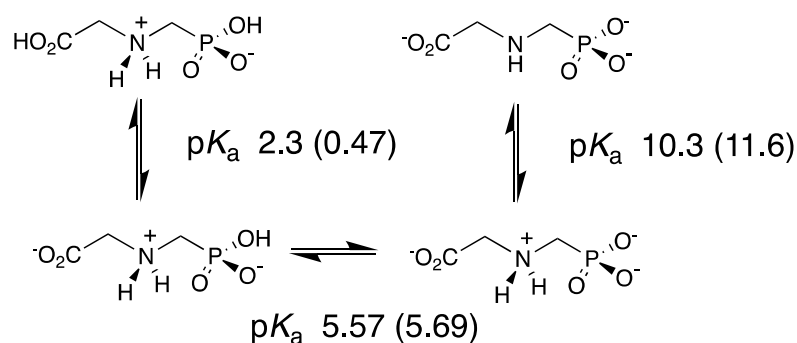
Scheme 4 Experimental 21 (0.1 M NaCl) and, in parentheses, the corresponding calculated 22 ( I = 0 ) pK_a values for glyphosate.
