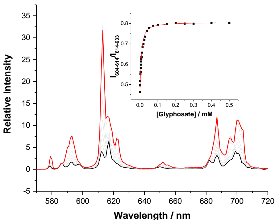
Figure 3 Changes in the emission intensity of [Eu.L 1 ] ( black ) (6 \mu M complex, 0.1 M NaCl, 0.1 M MES, pH 5.9, 295 K, \lambda_{\text{ex}} 365 nm) with incremental addition of glyphosate ( red ). The inset shows the variation of the emission intensity ratio (604-614/614-633 nm) as a function of increasing glyphosate concentration.
