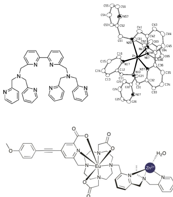
Scheme 6 ( upper ) Molecular structure of the 'BTPA' ligand and its complex with Zn 2+ . 33 and ( lower ) a possible binding motif for Zn 2+ in its complex with [EuL 2 ], showing 1:1 complexation (other ligands or a water molecule may be bound to the zinc ion, including a bridging carboxylate oxygen of the nearby macrocyclic moiety).
