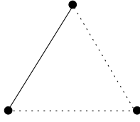
FIGURE 8. Completing a weighted graph with three vertices to form a cycle. The solid edge corresponds to orbits with non-trivial finite cyclic isotropy, while the dotted edges correspond to principal orbits.
