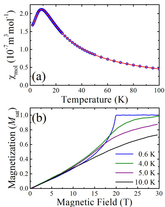
Fig. 2 (a) Molar susceptibility ( \chi_{\text{mol}} ) vs. temperature for 2 shows a broad maximum at 9 K. (b) Magnetization in units of the saturation magnetization ( M_{\text{sat}} ) vs magnetic field provided by a short-pulse magnet. Down sweeps of the magnetic field at various temperatures are shown. Data at 0.6 K are typical of well-isolated S = 1/2 antiferromagnetic chains.
