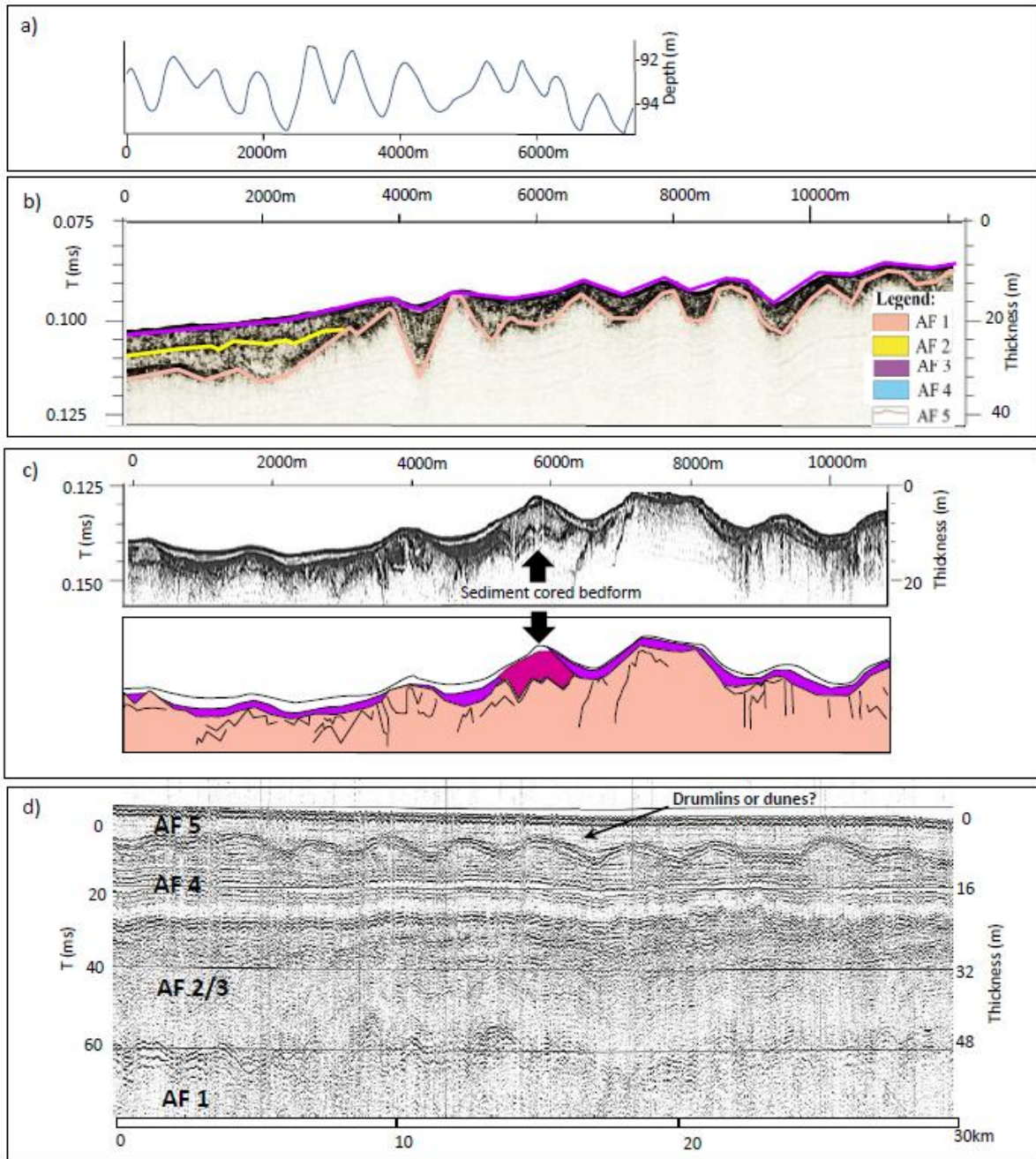
Fig. 11. a) A bathymetry cross profile across a series of mega-scale glacial lineations. Drift/bedrock cores not differentiated. b) Partially buried bedrock ridges. Where drift is slightly thicker their surface form is more subdued. c) In some localities glaciogenic sediment constitutes the whole bedform forming drumlins (pink = bedrock; purple = diamict AF3; fuschia = drift drumlin core. d) BGS seismic line 1993-1/1 close to the Northumberland coast. Note the buried streamlined bedforms. They have drumlin-like dimensions but have been previously interpreted as buried dunes by Brew (1996).
