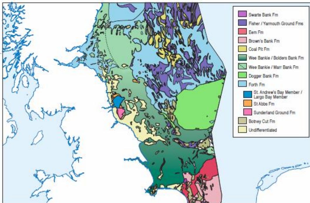
Fig. 2. a) The bedrock geology of the floor of the central western North Sea. Close to the Durham coast. Carboniferous, Permian and Triassic rocks are prevalent. b) The drift geology of the central western North Sea. Note the distribution of the Wee Bankie and Bolders Bank Formations which delimit the footprint of the North Sea Lobe.
