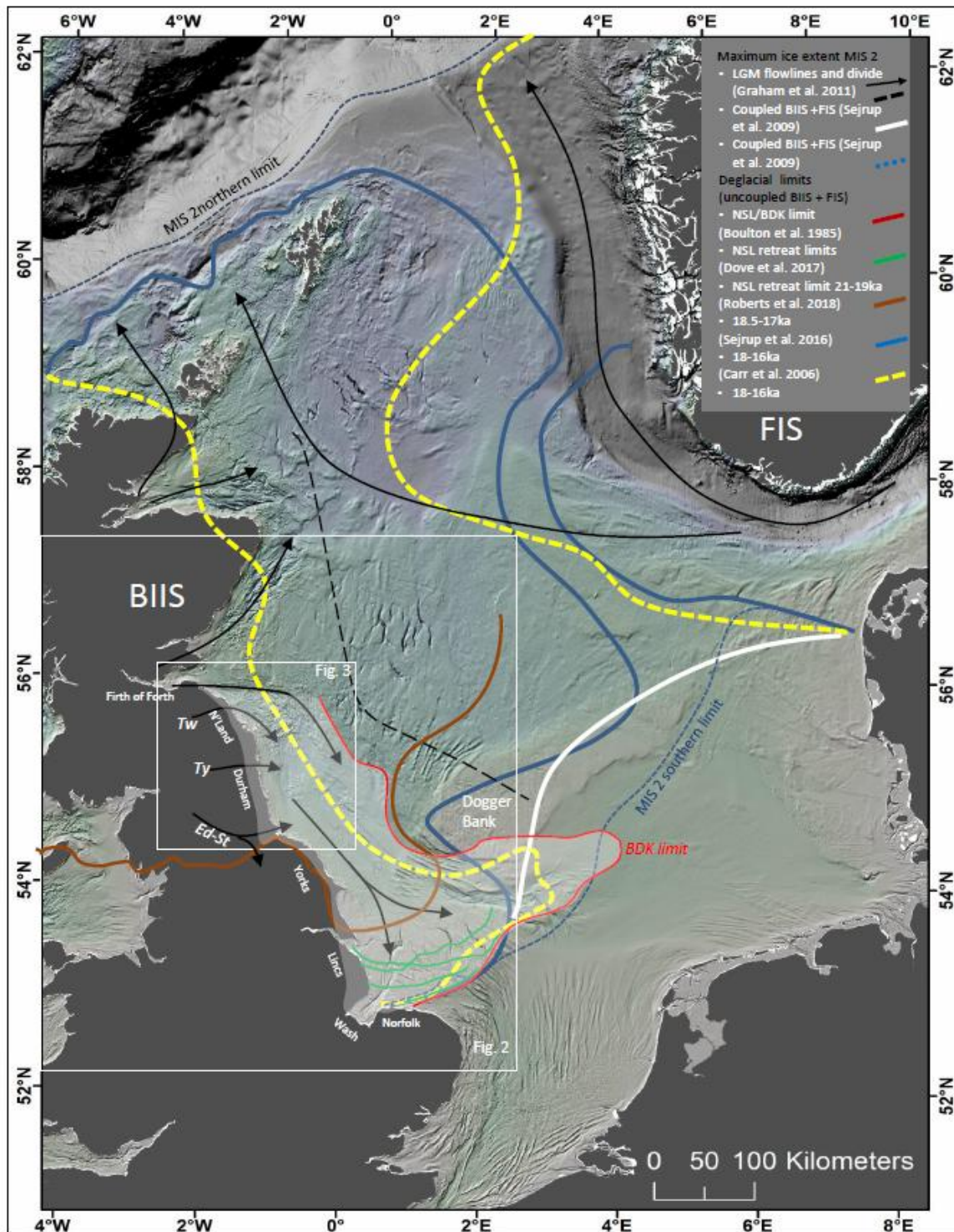
Fig. 1. A bathymetric overview of the North Sea showing the position of BIIS and FIS ice margins, flowlines and ice divides during MIS 2 glaciation. The NSL was distinctive lobe of ice that flowed southeast from the Firth of Forth region towards Norfolk in eastern England towards the end of MIS 2 glaciation. Its seafloor imprint has often been correlated to the distribution of Bolders Bank Formation (BDK) sediment, but controls on its hypsometry, dynamic behaviour and recession are poorly constrained. Major drainage basins feeding the NSL include the Firth of Forth, Tweed (Tw), Tyne Gap (Ty) and the Eden-Stainmore (Ed-St) gap (Image based on reconstruction of Dove et al., 2017 and Roberts et al. 2018).
