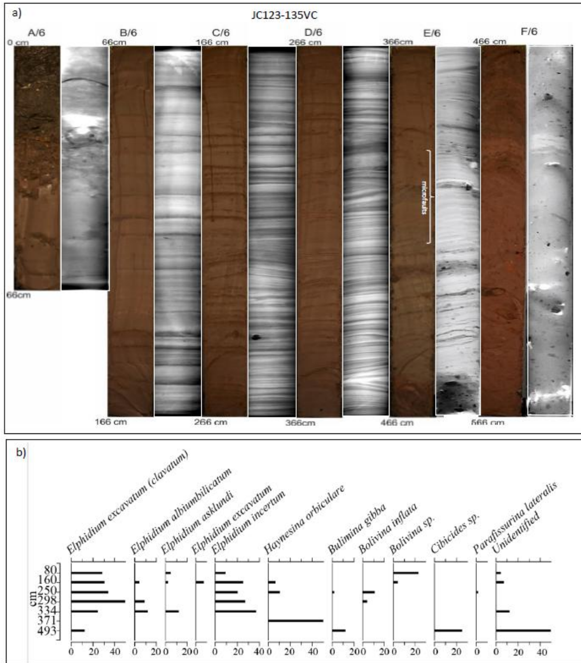
Fig. 8. a) Core JC123-135VC with paired photographs and X-ray images. This core typifies many in the study area with a lower massive diamict (AF3) grading upwards into a stratified diamict before the sediments become intensely laminated (AF4). The lack of clasts in the laminated sediments suggest a lack of ice rated input during deglaciation. The core is capped by a distinctive sandy/shelly deposit (AF5). b) Foraminiferal counts from core JC123-135VC. Elphidium excavatum (clavatum) and Cassidulina reniforme are known indicators of extreme glacial marine environments, and other indicator species such as Elphidium incertum , Elphidium asklundi , Elphidium albumbilicatum , Haynesina orbiculare and Bolivina sp. further corroborate cold glaciomarine conditions.
