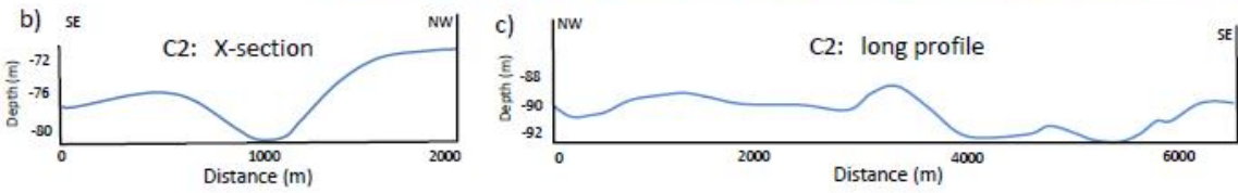
Fig. 13. a-c) Distinctive channels cut into bedrock in the northern part of the study area running NW to SE (parallel to former ice flow direction). C3 – C5 are anastomosing and interconnected. C2 is up to 10 m deep and has an up/down long profile.
