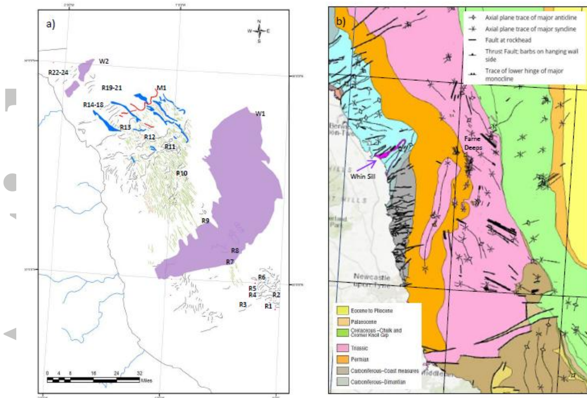
Fig. 14. The bedrock geology offshore from Durham/Northumberland showing the structural geology of the region compared to the distribution of glacial landforms. Transverse bedrock ridges trending NE to SW are prominent across the seafloor and formed in Carboniferous, Permian and Triassic rocks. They are controlled by orientation of synclines, faults or regional igneous intrusions. MSGL occur mainly occur Permian and Triassic bedrock but the juxtaposition of both bedrock-cored and sediment-cored bedforms reinforces the notion that in areas of thin sediment cover the subglacial bed is partially emergent and partially inherited with bedforms evolving via a combination of erosion, deposition and deformation.
