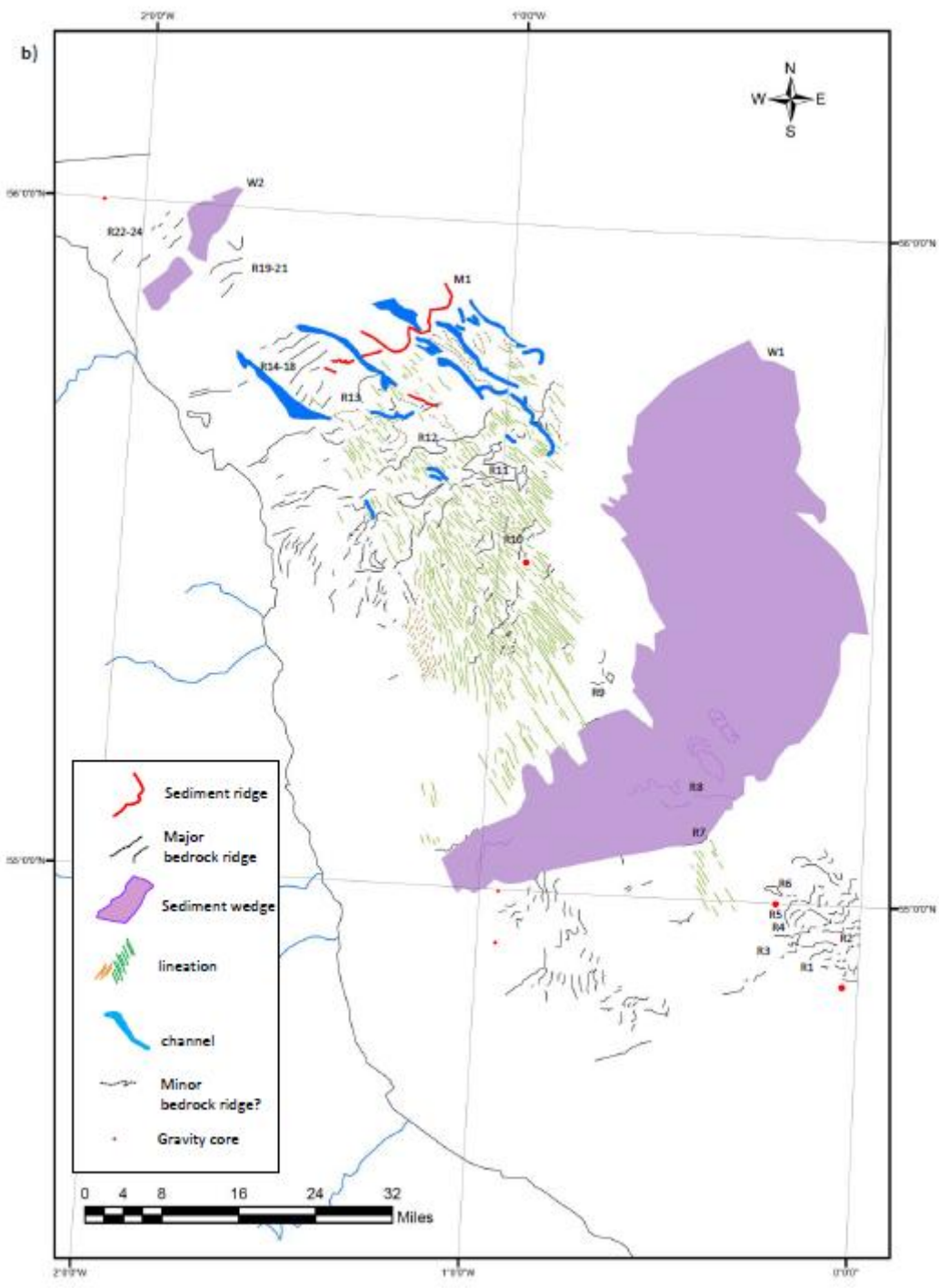
Fig. 3. a) The bathymetry of the central western North Sea close to the north east coast of England. The areas immediately offshore between Seaham and Eyemouth are very shallow but deepen to 113m in the central study area. b) Several distinctive landforms can be mapped across the seafloor. They include sediment wedges and ridges, lineations, channels and bedrock ridges.
