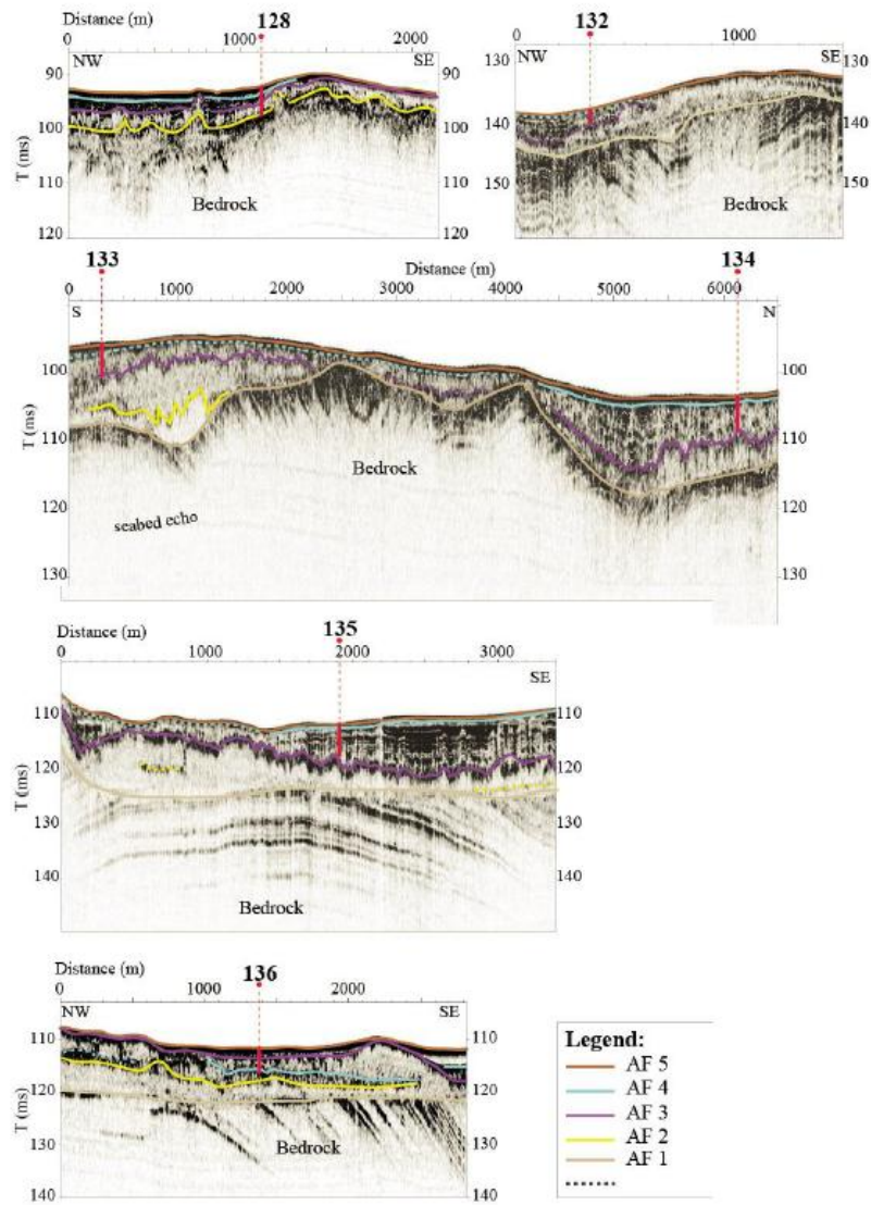
Fig. 6. Acoustic facies mapped at each core location. Most cores penetrate AF4 but only just reach AF3.
