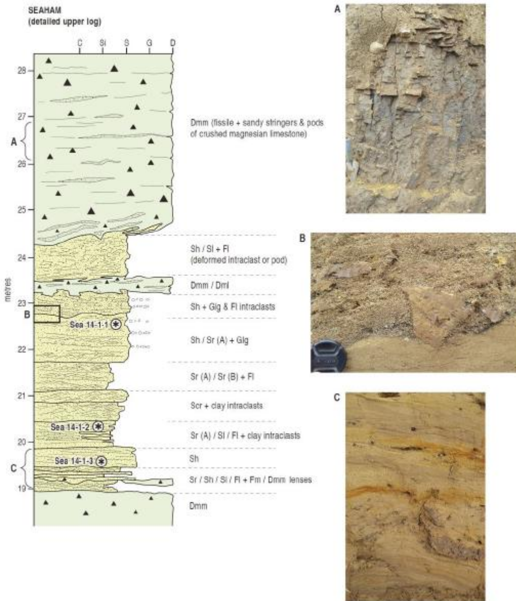
Fig. 10. The glacial stratigraphy from a coastal section at Seaham, County Durham. The section has two glacial diamicts separated by a glacial fluvial sand. These sediments cannot be directly related to the offshore acoustic stratigraphy as the near shore areas have been scoured of glacial sediment, but glaciofluvial sands provide three OSL ages that limit final deglaciation of the coast by the NSL to after 19.6 ka.
