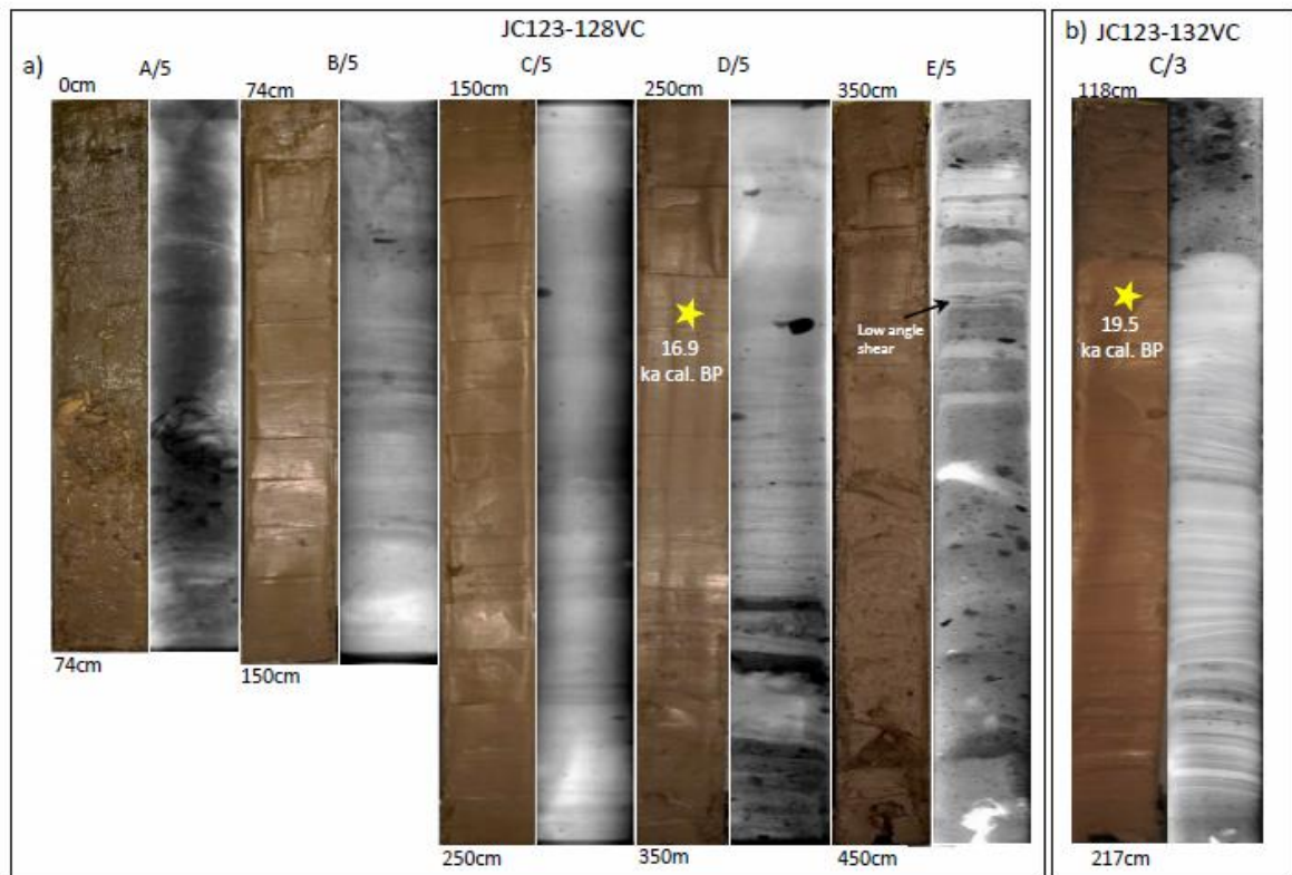
Fig. 7. a) Core JC123-128VC with paired photographs and X-ray images. The base of the core is diamictic (AF3) but grades upwards in to a laminated clay/silt with a decreasing in clast content (AF4). It is capped by a sandy/shelly deposit (AF5). A radiocarbon date from 280cm down core provided an age of 16.9 ka cal. BP. b) Core123-132VC; The lower laminated sediments in this core (AF4) provide at radiocarbon age of 19.5 ka cal. BP. They are truncated by a massive diamict mid core before grading back into AF4.
