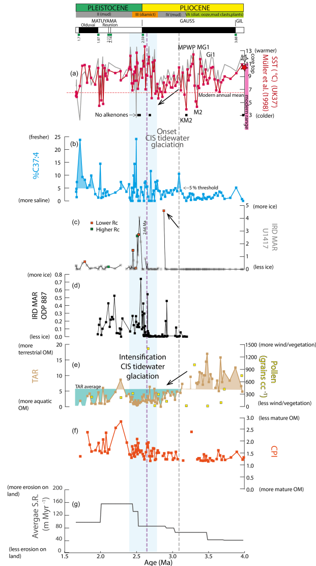
Figure 2. Site U1417 across the Pliocene–Pleistocene transition. (a) Red line: SST from U_{37}^{K'} index according to Müller et al. (1998) calibration; grey line: SST from U_{37}^K index according to PrahI et al. (1988) calibration. Black squares are samples in which alkenones were not detected. Dashed red line: modern averaged decadal (1955–2012) annual statistical mean SST of 6.4 °C at 0 m of water depth (NOAA WOA13; Boyer et al., 2013) at Site U1417, similar to the modern annual average SST of 7 °C at GAK1 station during the 1970–2018 time intervals for the 0–100 m water column depth (Weingartner et al., 2016) in the Gulf of Alaska; red star on the y axis: value of our youngest sample analysed at Site U1417 (U1417D 1H-1W 44-48; 0.016 Ma; SST = 10.6 °C with Müller et al., 1998, calibration; SST = 11.8 °C with PrahI et al., 1988, calibration); pink rectangle on the y axis: modern averaged decadal (1955–2012) statistical mean SST during winter and summer at Site U1417 and 0 m of water depth: 0–11.3 °C (NOAA WOA13; Boyer et al., 2013). (b) Abundance of the cold and/or freshwater alkenone C_{37:4} (%). The horizontal line shows the threshold of Bendle et al. (2005), above which subarctic–subpolar water masses were determined for the Nordic Seas. (c) IRD MAR ( g\ cm^{-2}\ kyr^{-1} ). Orange and green squares reflect the lower and higher average roughness coefficient (Rc) of the IRD quartz grains, respectively. (d) IRD MAR ( g\ cm^{-2}\ kyr^{-1} ) at ODP 887 (Prueher and Rea, 2001). (e) Terrestrial–aquatic n -alkane index (TAR, defined in the main text); the horizontal line shows the average TAR value for the study interval, and yellow squares represent pollen grain concentrations in grains per cubic centimetre. (f) CPI (defined in the main text). (g) Average sedimentation rates (see Fig. S3b; m\ Myr^{-1} ). Upper panel: Pliocene–Pleistocene boundary, magnetostratigraphy events and interpretations (see Figs. S2 and S3), and lithostratigraphic units of Site U1417 with simplified lithology (orange: ice-rafted diamict interbedded with mud; brown: marine mud; green: diatom ooze interbedded with debris flow deposits containing mud clasts and plant fragments) (Jaeger et al., 2014). The grey vertical line represents the onset of the Cordilleran Ice Sheet (CIS) glaciation (or oNHG) climate transition at 3 Ma; blue shading represents the 2.7–2.4 Ma climate transition with the intensification of the CIS tidewater glaciation (or iNHG) as in Table 1. The purple vertical line represents the onset of the Cordilleran Ice Sheet at the lower Klondike Valley, Yukon interior (Hidy et al., 2013; Fig. 1). Missing TAR or CPI data points are either a result of samples analysed for SSTs at the early stages of the project, which were not subsequently analysed for n -alkane distributions, or the result of samples in which chromatograms reflected poorly resolved n -alkane peaks.
