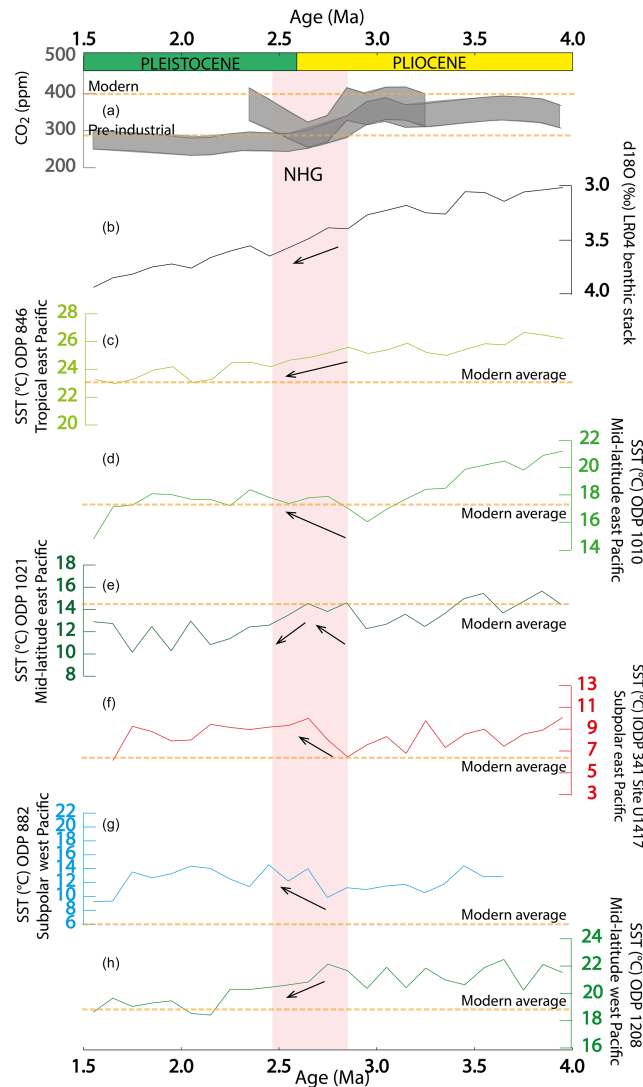
Figure 3. Pliocene–Pleistocene SST across the North Pacific. (a) Alkenone \delta^{13}\text{C} atmospheric \text{CO}_2 upper- and lower-end (ppm) estimates at Site ODP 999A (Seki et al., 2010b, revised in Foster et al., 2017) (4.0–1.5 Ma) and marine \delta^{11}\text{B} atmospheric \text{CO}_2 upper- and lower-end (ppm) estimates at Site ODP 999 (2.3–3.2 Ma) (Martínez-Botí et al., 2015, revised in Foster et al., 2017). (b) \delta^{18}\text{O} (‰) LR04 benthic stack (Lisiecki and Raymo, 2005). Alkenone SST ( ^{\circ}\text{C} ) from (c) ODP Site 846 (Herbert et al., 2017), (d) Site 1010 (Herbert et al., 2018a), (e) Site 1021 (Herbert et al., 2018b), (f) IODP Expedition 341 Site U1417 (Sánchez-Montes et al., 2019), (g) ODP Site 882 (Martínez-García et al., 2010b), and (h) ODP Site 1208 (Herbert et al., 2018c). The SST records are arranged from top to bottom following an anticlockwise direction from tropical east to subpolar east, subpolar west, and tropical west locations. Orange horizontal lines indicate reference levels of pre-industrial times and/or modern values for each of the records or sites (SSTs from NOAA WOA13, Boyer et al., 2013). Arrows indicate cooling or warming trends across the oNHG in the Pacific Ocean. All records are 1 kyr linearly interpolated and 100 kyr smoothed. Ages (Ma) have been determined through the calculation of the mean for each interval.
