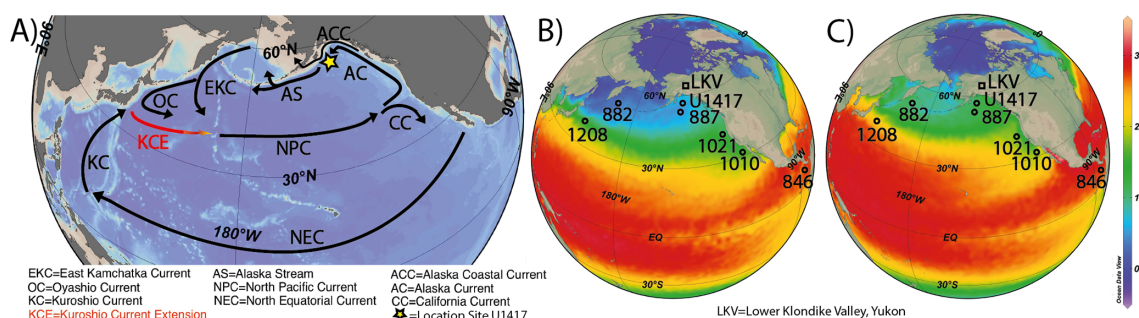
Figure 1. Map of modern ocean circulation and SSTs. (a) Modern North Pacific Ocean circulation, (b) December and (c) September 1955–2013 SST average centred in the North Pacific Ocean (NOAA WOA13; Locarnini et al., 2013), and core and sample sites discussed in this study. Map made using Ocean Data View (Schlitzer, 2018).
