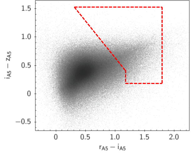
Figure 4. Our \bar{z} = 0.68 LRG photometric selection, following the colour cuts of Ross et al. (2008) used in the selection of the AAOmega LRG sample. The objects shown here are classified as galaxies based on their VST ATLAS i-band morphological classification and lie within a magnitude limit of 19.8 < i_{Kron} < 20.5 .
