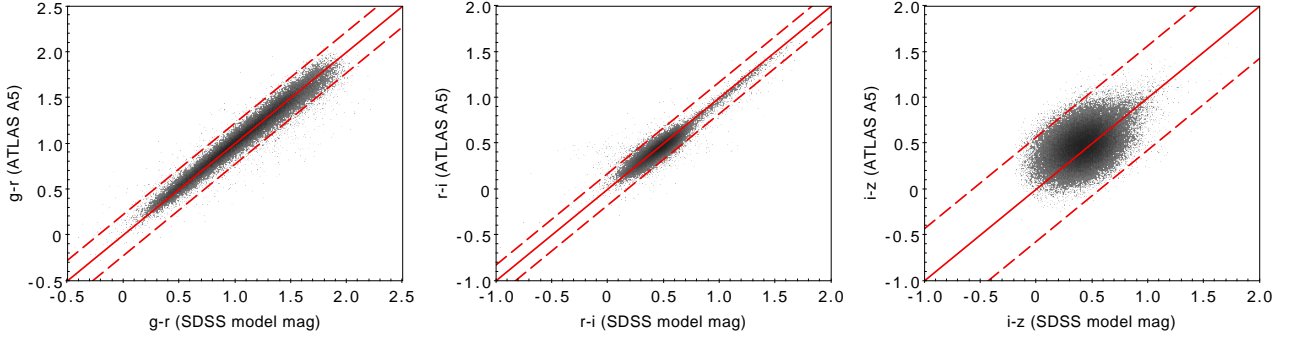
Figure A1. A comparison of the g-r , r-i and i-z colours based on VST ATLAS Aperture 5 and SDSS model magnitudes. Given the similarity between the colours, we use the SDSS cuts in our LRG sample selections, described in Section 2.2. Here the dashed lines indicate the 3\sigma outliers.
