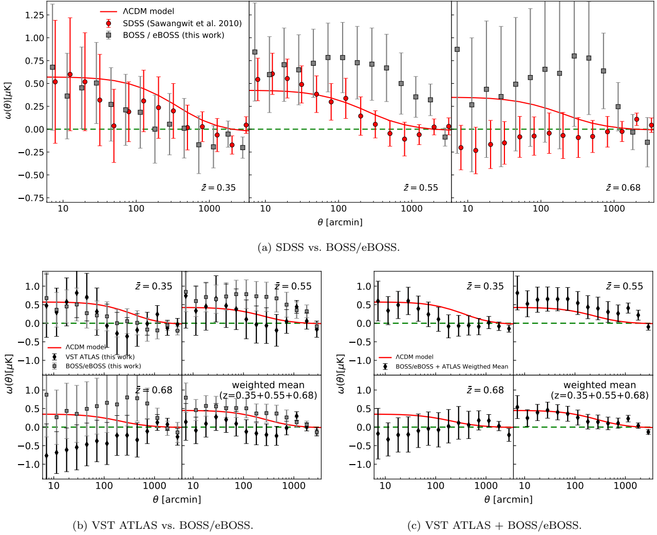
Figure 9. (a) Comparison of the SDSS and BOSS/eBOSS ISW measurements. (b, c) same as (7a, 7b) but comparing / combining the VST ATLAS ISW measurements to those based on BOSS/eBOSS.
