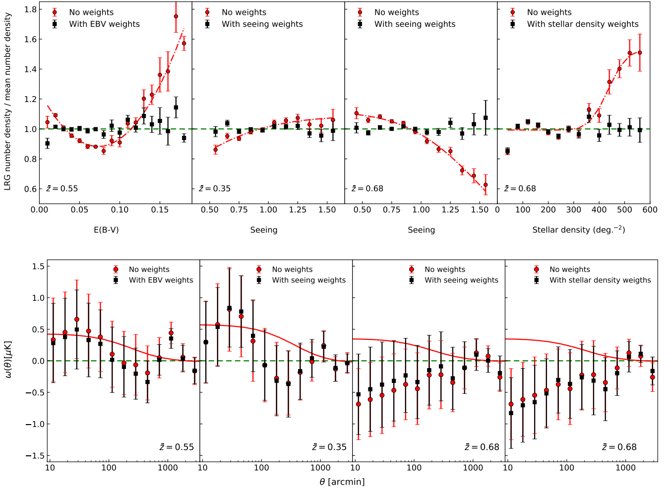
Figure B1. Top panel: Normalised projected LRG number density as a function of Galactic extinction (in E(B-V) ), seeing (in r -band for \bar{z} = 0.35 and i -band for \bar{z} = 0.68 ) and projected stellar density (limited to 19.8 < i < 20.5 corresponding to the magnitude limits of the \bar{z} = 0.68 LRG sample). Here the dot-dashed curves are the best-fit relationships used to define the weights correcting for the observed systematic trends. Bottom panel: The impact of including the E(B-V) , seeing and stellar density weights from the top panel on our ISW measurements. In all cases, the inclusion of weights do not appear to have a significant impact on our ISW measurements.
