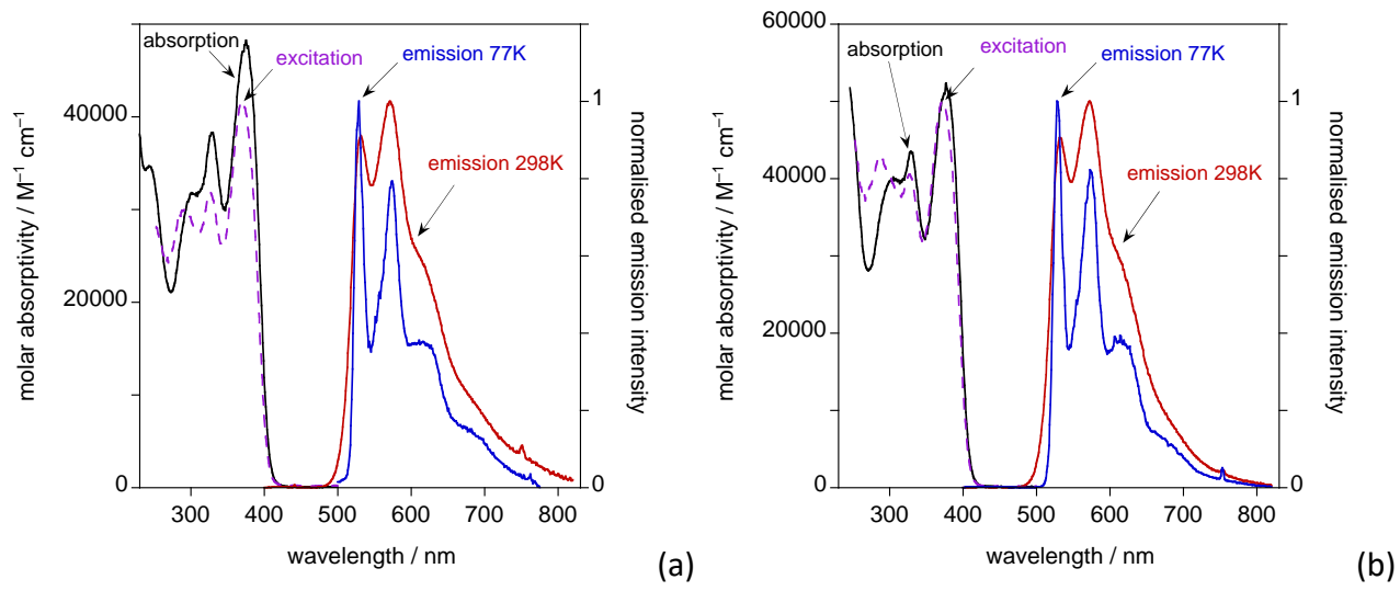
Figure 13: Absorption (black line), excitation (dashed purple) and emission (red) spectra of: (a) of complex 4 in CH_2Cl_2 at 298 K and its emission spectrum in EPA at 77 K (blue) and (b) complex 5 in CH_2Cl_2 at 298 K and its emission spectrum in EPA at 77 K (blue).
