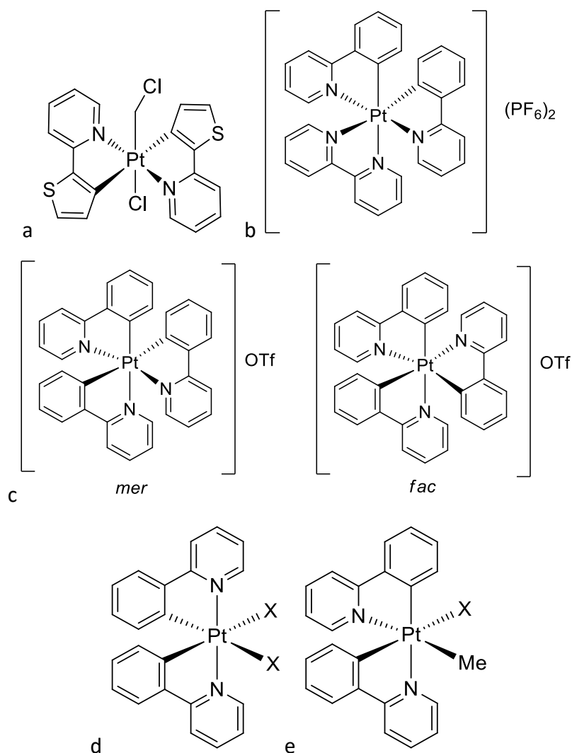
Figure 1: Model structures from a) Chassot et al. [7] who reported a platinum(IV) system with 2-(2-thienyl)pyridine ligands after the oxidative addition of \text{CH}_2\text{Cl}_2 ; b) Jenkins and Bernhard [8] showing the [\text{Pt}(\text{C}^{\wedge}\text{N})_2(\text{N}^{\wedge}\text{N})]^+ base unit, with reported functionalisation of both the \text{C}^{\wedge}\text{N} and \text{N}^{\wedge}\text{N} rings with fluorine and methoxy groups; c) the mer and fac isomers of the base unit of tris(cyclometallated)platinum(IV) complexes reported by Juliá et al. [6b] , with reported functionalisation of the \text{C}^{\wedge}\text{N} rings with fluorine and methyl groups, as well as systems where the pyridyl ring is replaced with pyrazole; Juliá et al. [9a] showing d) symmetric and e) asymmetric bis-cyclometallated 2-phenylpyridine systems, where \text{X} = \text{F}, \text{Cl}, \text{Br}, \text{I}, \text{OTf}, \text{OAc}, \text{TFA} .
