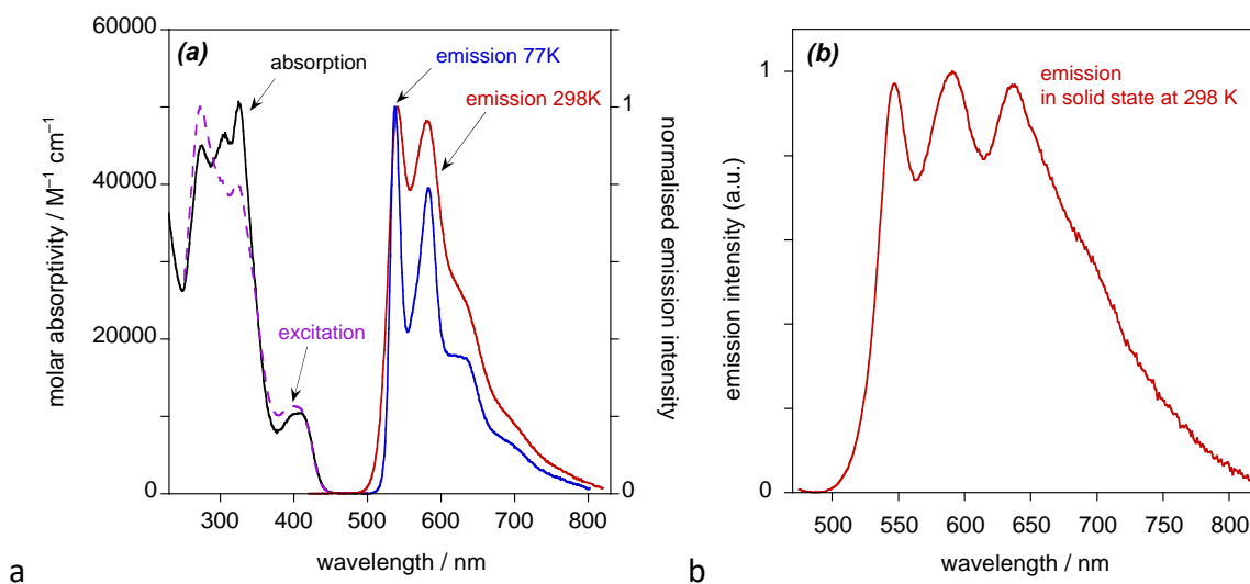
Figure 11: (a) Absorption (black line), excitation (dashed purple) and emission (red) spectra of complex 3 in CH_2Cl_2 at 298 K and the emission spectrum in EPA at 77 K (blue). (b) The emission spectrum of powdered 3 at 298 K.
