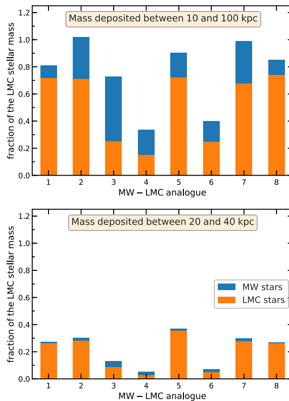
Figure 4. The increase in the stellar halo mass expressed as a fraction of the stellar mass of the LMC analogue. Plotted is the mass deposited in the stellar halo between 10 and 100 kpc (top panel) and between 20 and 40 kpc (bottom panel). The increase due both to stars that were initially part of the LMC analogue (orange) and to stars that were initially part of MW analogue (blue) is shown. Each column corresponds to a MW–LMC analogue, in the same order as in Fig. 3.
