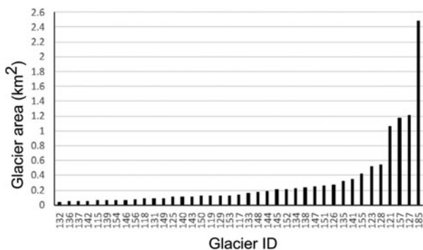
Fig. 3. Overview of glacier size distribution within the study site (see Fig. 1) as recorded in the NGI. Only 10% of glaciers are >1 \text{ km}^2 while 85% of glaciers are \leq 0.5 \text{ km}^2 .
