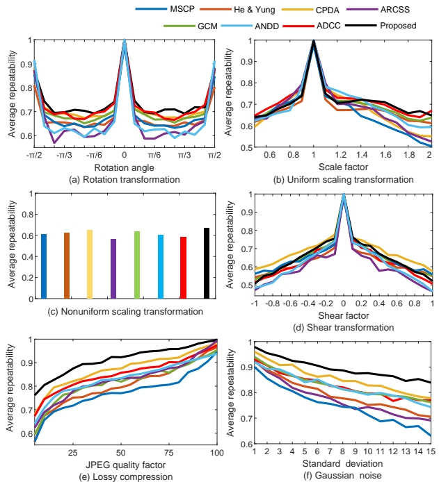
Fig. 13 Average repeatability of the eight detectors under rotation, uniform scaling, non-uniform scaling, shear transforms, lossy JPEG compression, and additive white Gaussian noises.
