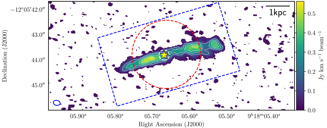
Figure 3. An integrated brightness map of \geq 3\sigma CO(2-1) emission in the Hydra-A brightest cluster galaxy. The brightness is integrated from -500 \text{ km s}^{-1} to +500 \text{ km s}^{-1} about the galaxy’s systemic velocity. Contours marking 0.15, 0.25, 0.35 and 0.45 \text{ Jy km s}^{-1} \text{ beam}^{-1} emission are shown in white. The yellow star indicates the position of the mm-continuum source while the large, dashed blue box and dashed white circle indicate the respective regions from which the spectra in Fig. 2 and 6 are extracted. The large, dashed red circle, which is approximately the same size as the CO(1-0) beam, indicates the region from which the spectra in Fig. 8 are extracted. The CO(2-1) beam size is shown in blue in the bottom-left corner.
