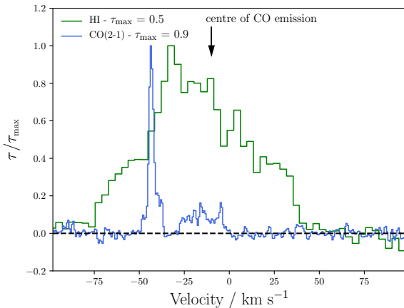
Figure 7. Hydra-A’s normalized CO(2-1) and HI optical depth profiles for the region co-spatial with the mm-continuum source. The CO(2-1) optical depth profile is produced using the spectrum shown in the right panel of Fig. 6, and the HI profile is taken from VLBA observations presented in Taylor (1996).
