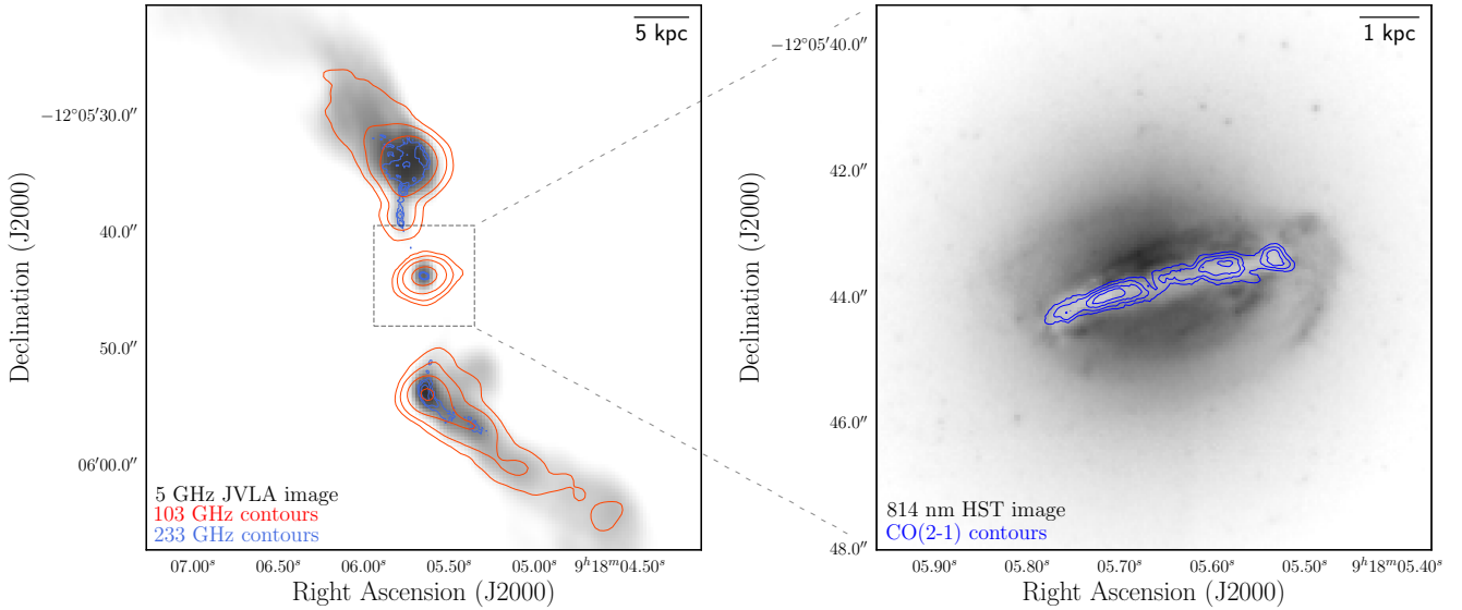
Figure 1. Left: A 5GHz Karl G. Jansky Very Large Array (VLA) radio image of Hydra-A showing powerful radio lobes emanating from the centre of the brightest cluster galaxy, with 0.19 \text{ arcsec pixel}^{-1} resolution (Project 13B-088). Contours of our 233 GHz ALMA continuum image are overlaid in blue and lower angular resolution 103 GHz contours are shown in red. Right: Contours from a CO(2-1) integrated brightness map (described in §3), which mark the 0.15, 0.25, 0.35 and 0.45 \text{mJy beam}^{-1} emission regions, overlaid onto a F814W Hubble Space Telescope (HST) near-infrared image of the brightest cluster galaxy (Mittal et al. 2015), with a resolution of 0.05 \text{ arcsec pixel}^{-1} . This highlights how the galaxy’s dust lane, which is opaque to optical wavelengths, is spatially coincident with a molecular gas disc.
