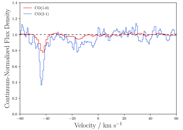
Figure 8. Hydra-A’s continuum-normalized CO(1-0) and CO(2-1) flux density after the removal of the emission which is seen across the galaxy’s disc. These spectra are both extracted from the region indicated by the large, dashed red circle in Fig. 3. A wider region is used to extract these spectra due to the larger beam size of the CO(1-0) images. By comparing the strength of the absorption seen for the two lines, we find that the absorbing gas has a temperature of T_{\text{ex}} = 42^{+25}_{-11} K and line-of-sight column densities of N_{\text{CO}} = 2^{+3}_{-1} \times 10^{17} \text{cm}^{-2} and N_{\text{H}_2} = 7^{+10}_{-4} \times 10^{20} \text{cm}^{-2} .
