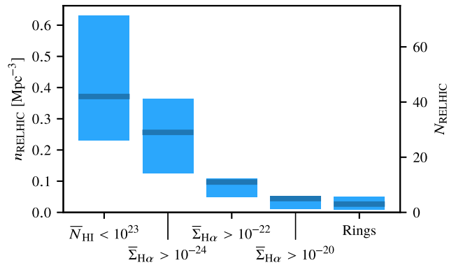
Figure 7. Number density distribution of H \alpha -fluorescent haloes in APOSTLE. The median values are shown by thick solid lines; shaded regions indicate 10 th –90 th percentiles. From left to right, we show the number density of all RELHICs with H I column densities below our star formation threshold, those with surface brightnesses exceeding three different limiting values, and those with discernible ring-shaped surface brightness profiles. Here, N_{\text{H I}} \equiv N_{\text{H I}}/(\text{cm}^2) and \Sigma_{\text{H}\alpha} \equiv \Sigma_{\text{H}\alpha}/(\text{erg s}^{-1} \text{ cm}^{-2} \text{ arcsec}^{-2}) . The right-hand axis indicates the corresponding number counts per APOSTLE volume.
