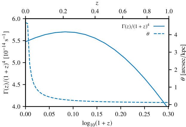
Figure 8. Redshift evolution of the apparent surface brightness (solid curve; left scale) and the angular separation corresponding to a comoving kpc (dashed curve; right scale).
