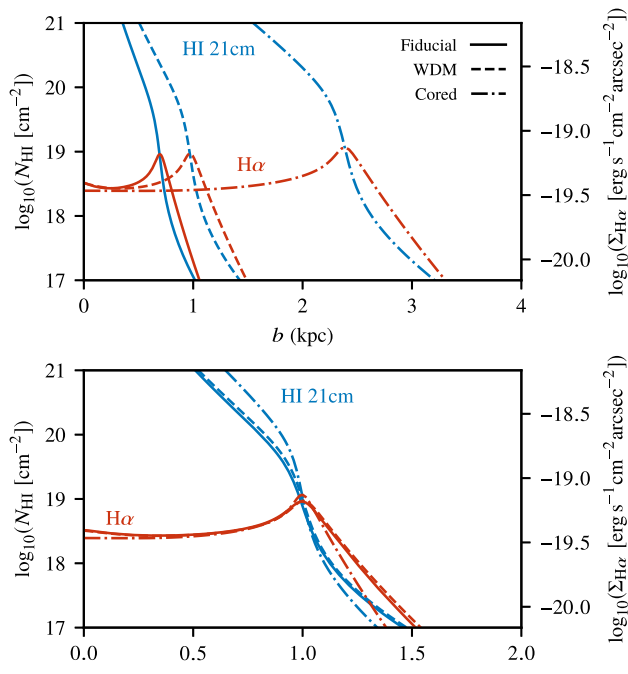
Figure 12. H I column density profiles (blue) for models with different dark matter density profiles, with corresponding H \alpha surface brightness profiles (red). Profiles are shown as a function of impact parameter b , both in physical units (top panel) and normalized by r_{\max} (bottom panel). For each model, profiles are shown for the most massive halo which satisfies our star formation criterion.
