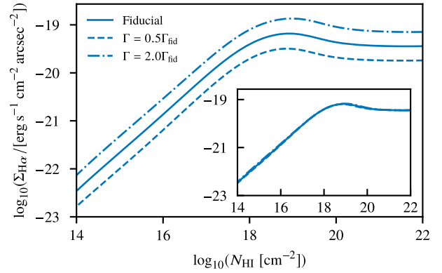
Figure 11. Surface brightness as a function of H I column density for different photoionization rates. In the inset panel, we show that the three N_{\text{HI}} - \Sigma_{\text{H}\alpha} relations are self-similar when the surface brightness is scaled by the ratio f_{\Gamma} = \Gamma / \Gamma_{\text{fid}} .
