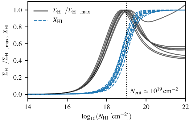
Figure 10. Normalized H \alpha surface brightness profiles for the most massive halo satisfying our star formation criterion in each model we consider (black), shown with corresponding H neutral fractions X_{\text{HI}} (dashed blue).
