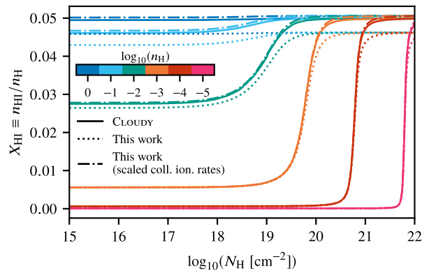
Figure B2. H I neutral fraction as a function of total H column density for isothermal, H-only plane-parallel models with T_{\text{gas}} = 20000 \text{ K} . Solid and dotted curves correspond to output generated by CLOUDY and our code, respectively, while the dot-dashed curves show our predictions if the collisional ionization rates we use are rescaled to match those in CLOUDY.
