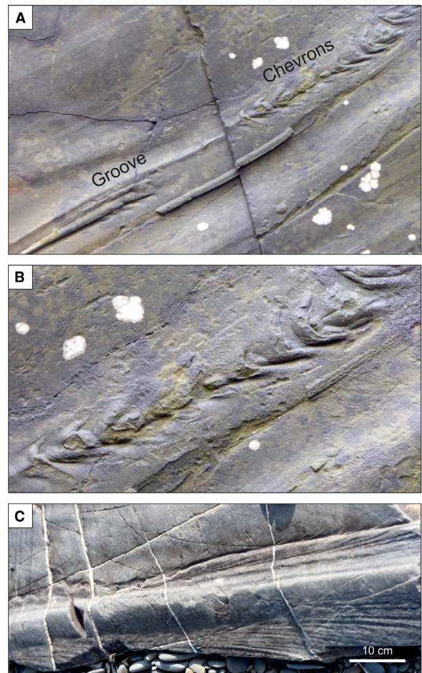
Fig. 13. Examples of chevrons. (A) Uninterrupted chevrons (ca 3 cm in width) changing downstream (to the left) into a groove mark (ca 1 cm in width). This suggests that a particle moved down through the flow until it started sliding along the bed, at which point it ceased to produce chevrons. (B) Close up of (A) showing detail of the uninterrupted chevrons. (A) and (B) From the Lower Silurian Aberystwyth Grits, Wales. (C) Interrupted chevrons, showing flow from right to left. From the middle Ordovician Cloridorme Formation, Gaspé Peninsula, Quebec, Canada.
