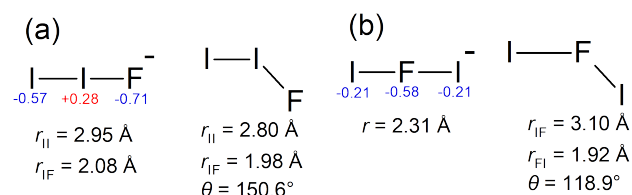
Fig. 4 Calculated equilibrium geometries at the CCSD(T)//def2-TZVPD level of theory for: (a) [\text{I-I-F}]^- and [\text{I-I-F}] , and (b) [\text{I-F-I}]^- and [\text{I-F-I}] . NBO charges (red and blue font) are given for the anions. The lowest energy isomer, [\text{I-I-F}]^- has C_{\infty h} symmetry, and [\text{I-I-F}] has C_s symmetry.
