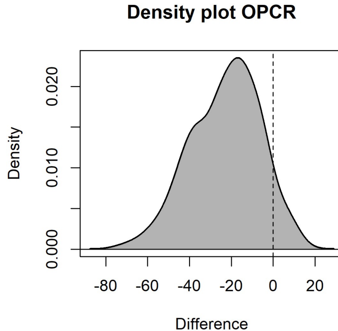
Fig 4. Density distributions of differences in OPCR values for a set of 216 individuals. Difference = OPCR_{Winchester\ et\ al.,\ 2014} - OPCR_{Berthaume\ et\ al.,\ 2019} . 93.5% of the OPCR values published here are higher than in [15]. https://doi.org/10.1371/journal.pone.0215436.g004
