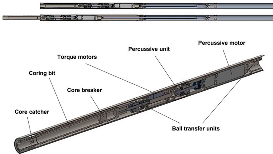
Fig. 13. The P-RAID unit in stowed (top) and full drill extension (below) configurations. Note that the entire stack is around 3.5 m long, and would be mounted below the RAID itself. At bottom, a close-up of the travelling module inside the deployment barrel. The auger exists around the outside of the deployable coring bit.
