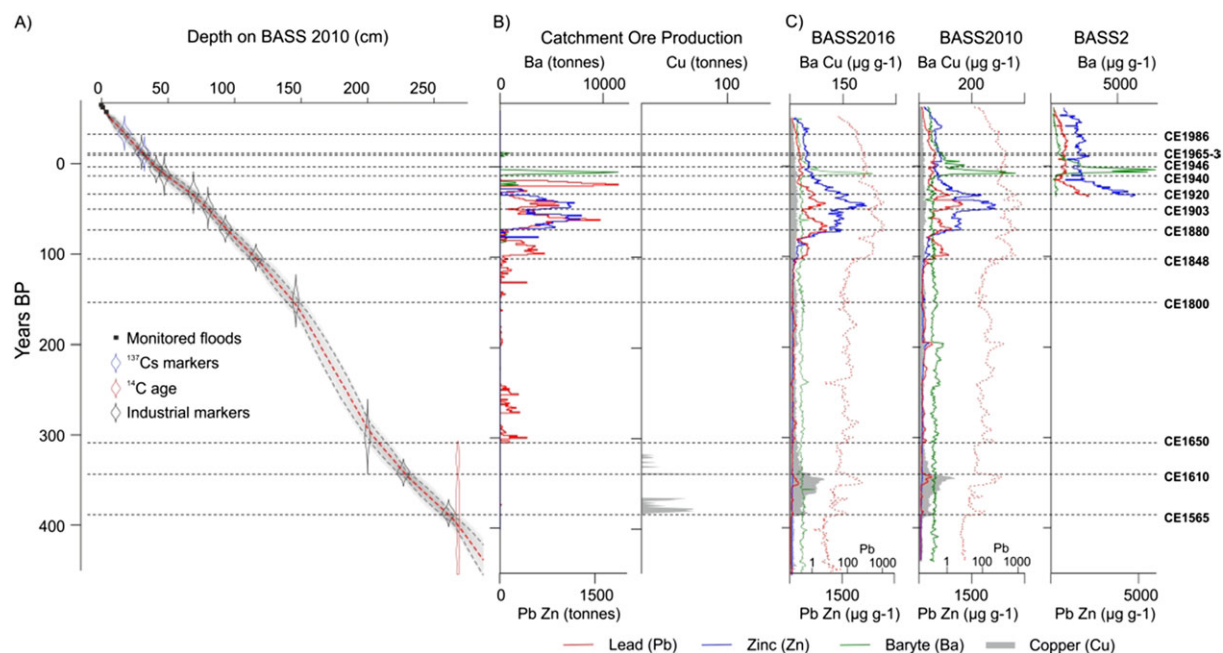
Figure 2. Age-depth information for Bassenthwaite Lake and the metal pollutant stratigraphy. A. Geochronological data and the Bayesian age-depth model for BASS-2010 showing the pollution markers, a ^{14}\text{C} age, markers for fallout radionuclides ( ^{137}\text{Cs} ) in 1963 and 1986, the modelled weighted mean age (red pecked line), the 2\sigma age probability (greyscale), and 2\sigma uncertainty age range (grey pecked lines). B. Metal ore production in tons from mines in the catchment (Tyler, 2003; Tyler, 2005a; Tyler, 2005b). C. Metal concentration data measured by XRF plotted against age derived from age-depth models for BASS-2016, BASS-2010 and BASS-2. Pb (solid red), Zn (blue), Ba (green) and Cu (grey fill). Pb is plotted for BASS-2016 and BASS-2010 with a log axis (red dashed line) to show patterns at lower concentrations. Time markers and their age extend across the plot (see Table I). [Colour figure can be viewed at wileyonlinelibrary.com ]
