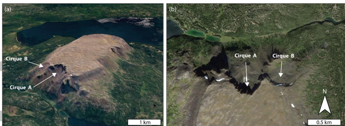
Fig. 8. Tuya Butte, northern British Columbia. (a) Landsat image viewed obliquely (from the northwest) in Google Earth™. (b) PlanetScope satellite image, clearly showing the two cirques (A = 59.136°N, 130.570°W; B = 59.137°N, 130.560°W) eroded into the tuya's northern flank.
