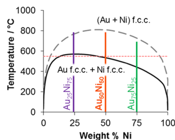
Figure 8. Phase diagram for Au–Ni alloying versus separate fcc phases as a function of composition (data taken from ref 17). The gray dashed line is the thermodynamic phase boundary in the bulk, and the solid black line is for a 13 nm nanoparticle. The horizontal dashed red line highlights the steady state reaction temperature of 550 °C, and the vertical lines indicate the bimetallic compositions used in this study (their nominal compositions are indicated, and the actual weight percent plotted is based on the ICP measured composition of the supported nanoparticles).
